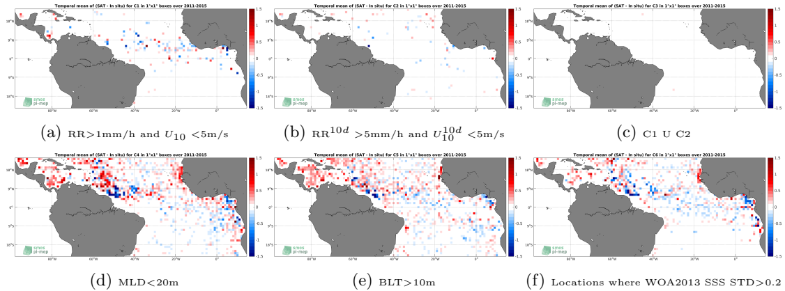
Figure 12: Temporal mean gridded over spatial boxes of size 1^\circ \times 1^\circ of \Delta SSS (Aquarius-L3-JPL-V5-MONTHLY - Argo) for 6 different subdatasets corresponding to: RR > 1\text{mm/h} and U_{10} < 5\text{m/s} (a), RR^{10d} > 5\text{mm/h} and U_{10}^{10d} < 5\text{m/s} (b), C1 U C2 (c), MLD < 20\text{m} (d), BLT > 10\text{m} (e), Locations where WOA2013 SSS STD > 0.2 (f).
