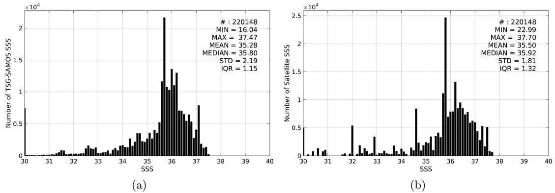
Figure 2: Histograms of SSS from TSG-SAMOS (a) and Aquarius-L3-JPL-V4-7DAY-RUNNING (b) considering all match-up pairs per bins of 0.1 over the Tropical Atlantic Ocean Pi-MEP region and for the full satellite product period.
