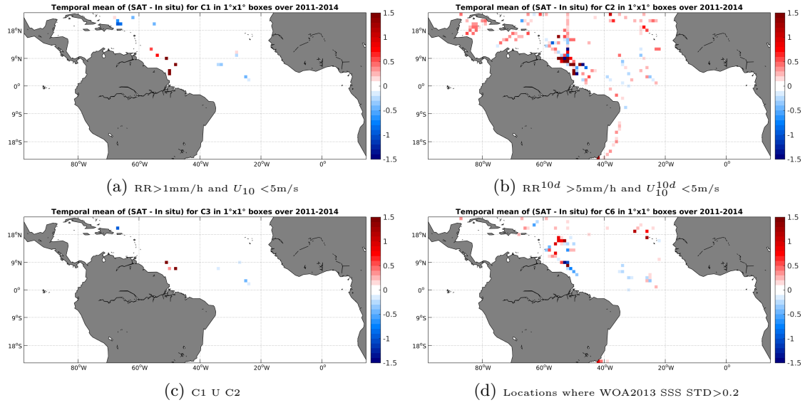
Figure 12: Temporal mean gridded over spatial boxes of size 1^\circ \times 1^\circ of \Delta SSS (Aquarius-L3-JPL-V4-7DAY-RUNNING - TSG-SAMOS) for 4 different subdatasets corresponding to: RR > 1 mm/h and U_{10} < 5 m/s (a), RR^{10d} > 5 mm/h and U_{10}^{10d} < 5 m/s (b), C1 U C2 (c), Locations where WOA2013 SSS STD > 0.2 (d).
