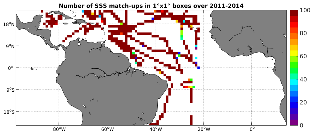
Figure 4: Number of SSS match-ups between TSG-SAMOS SSS and the Aquarius-L3-JPL-V4-7DAY-RUNNING SSS product for the Tropical Atlantic Ocean Pi-MEP region over 1^\circ \times 1^\circ boxes and for the full satellite product period.
