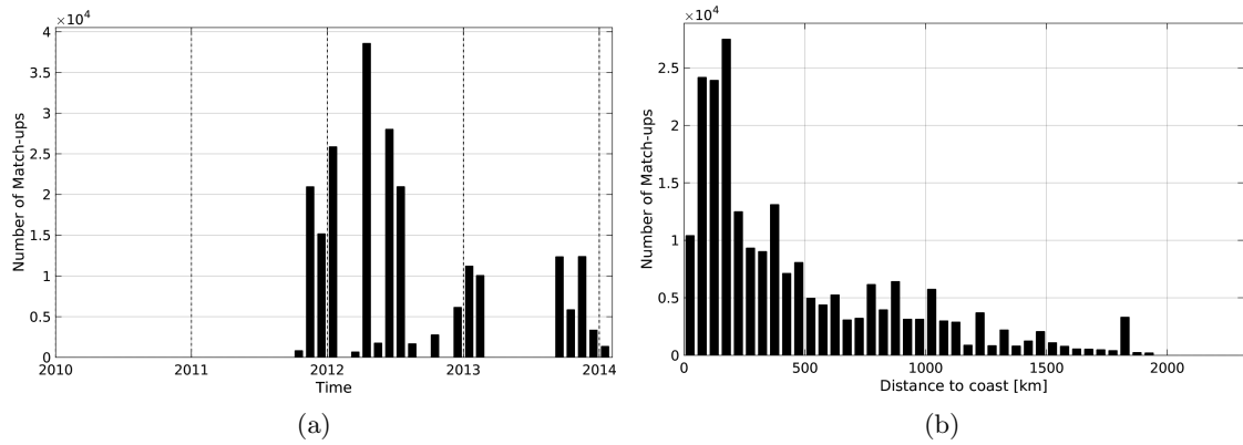
Figure 1: Number of match-ups between TSG-SAMOS and Aquarius-L3-JPL-V4-7DAY-RUNNING SSS as a function of time (a) and as function of the distance to coast (b) over the Tropical Atlantic Ocean Pi-MEP region and for the full satellite product period.
