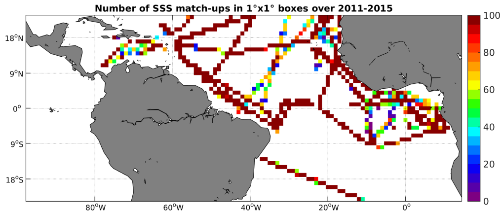
Figure 4: Number of SSS match-ups between TSG-GOSUD-Research-vessel SSS and the Aquarius-L3-JPL-V4-7DAY-RUNNING SSS product for the Tropical Atlantic Ocean Pi-MEP region over 1^\circ \times 1^\circ boxes and for the full satellite product period.
