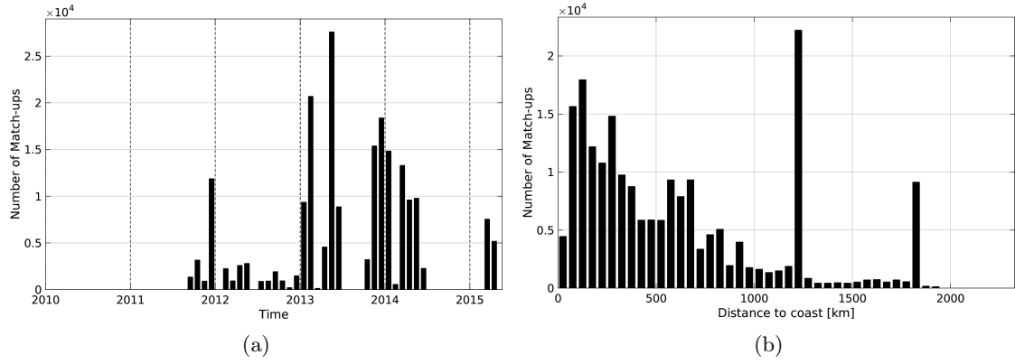
Figure 1: Number of match-ups between TSG-GOSUD-Research-vessel and Aquarius-L3-JPL-V4-7DAY-RUNNING SSS as a function of time (a) and as function of the distance to coast (b) over the Tropical Atlantic Ocean Pi-MEP region and for the full satellite product period.
