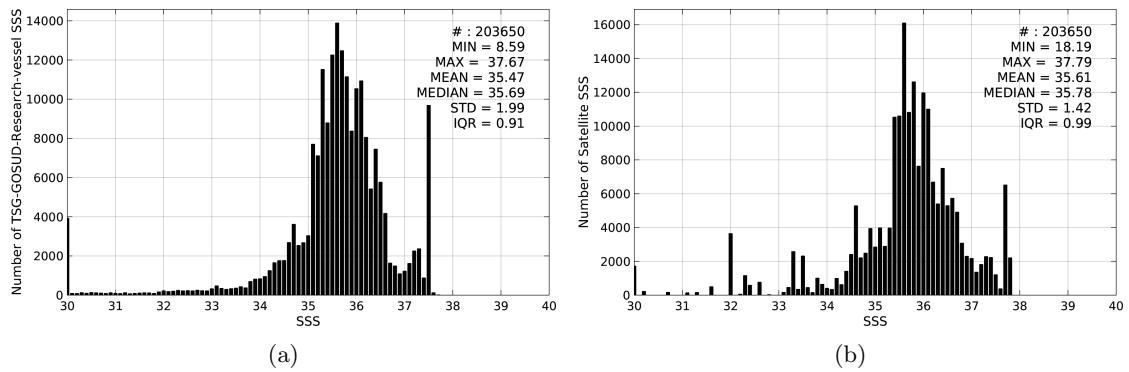
Figure 2: Histograms of SSS from TSG-GOSUD-Research-vessel (a) and Aquarius-L3-JPL-V4-7DAY-RUNNING (b) considering all match-up pairs per bins of 0.1 over the Tropical Atlantic Ocean Pi-MEP region and for the full satellite product period.
