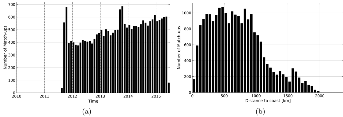
Figure 1: Number of match-ups between Argo and Aquarius-L3-JPL-V4-7DAY-RUNNING SSS as a function of time (a) and as function of the distance to coast (b) over the Tropical Atlantic Ocean Pi-MEP region and for the full satellite product period.
