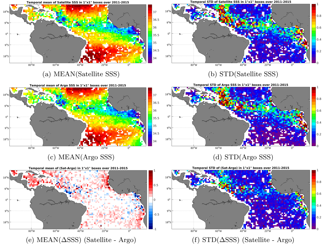
Figure 6: Temporal mean (left) and STD (right) of SSS from Aquarius-L3-JPL-V4-7DAY-RUNNING (top), Argo (middle), and of \Delta SSS (Satellite - Argo). Only match-up pairs are used to generate these maps.
