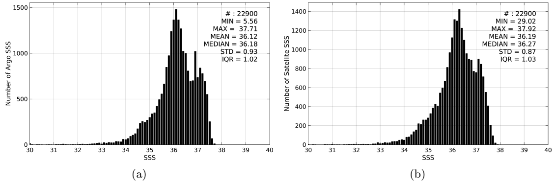
Figure 2: Histograms of SSS from Argo (a) and Aquarius-L3-JPL-V4-7DAY-RUNNING (b) considering all match-up pairs per bins of 0.1 over the Tropical Atlantic Ocean Pi-MEP region and for the full satellite product period.
