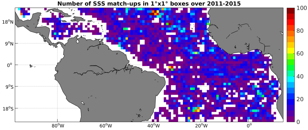
Figure 4: Number of SSS match-ups between Argo SSS and the Aquarius-L3-JPL-V4-7DAY-RUNNING SSS product for the Tropical Atlantic Ocean Pi-MEP region over 1^\circ \times 1^\circ boxes and for the full satellite product period.
