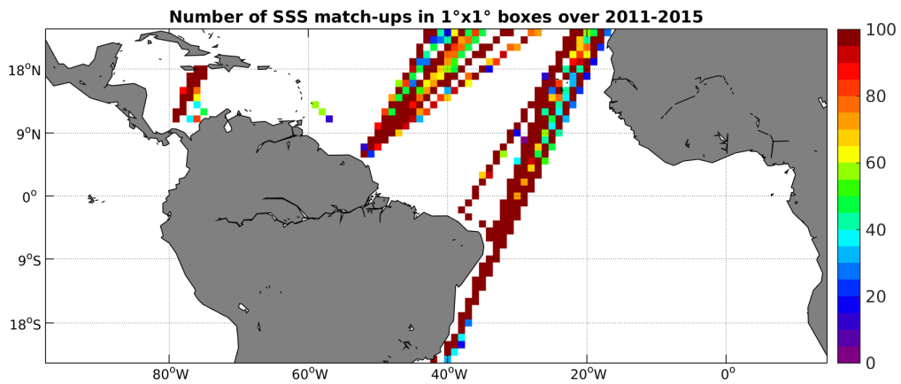
Figure 4: Number of SSS match-ups between TSG-LEGOS-DM SSS and the Aquarius-L3-JPL-V4-MONTHLY SSS product for the Tropical Atlantic Ocean Pi-MEP region over 1^\circ \times 1^\circ boxes and for the full satellite product period.
