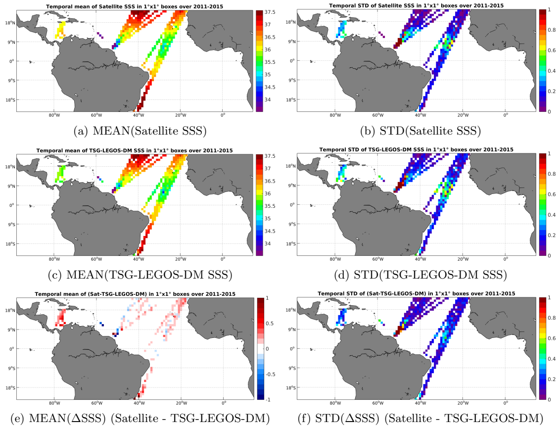
Figure 6: Temporal mean (left) and STD (right) of SSS from Aquarius-L3-JPL-V4-MONTHLY (top), TSG-LEGOS-DM (middle), and of \Delta SSS (Satellite - TSG-LEGOS-DM). Only match-up pairs are used to generate these maps.
