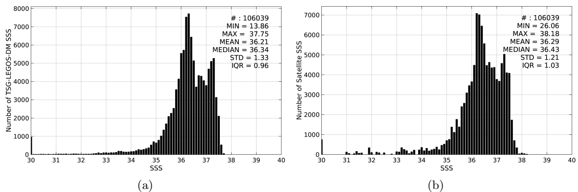
Figure 2: Histograms of SSS from TSG-LEGOS-DM (a) and Aquarius-L3-JPL-V4-MONTHLY (b) considering all match-up pairs per bins of 0.1 over the Tropical Atlantic Ocean Pi-MEP region and for the full satellite product period.
