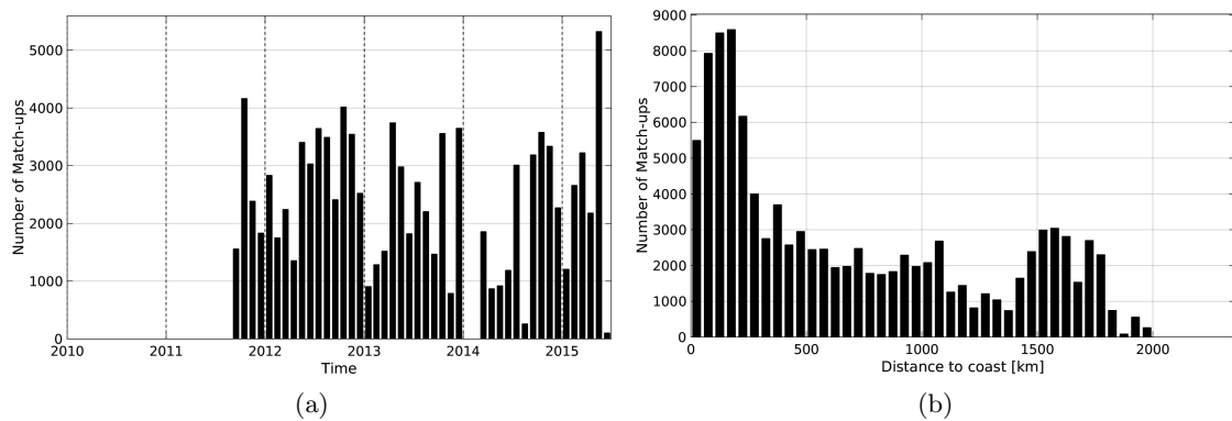
Figure 1: Number of match-ups between TSG-LEGOS-DM and Aquarius-L3-JPL-V4-MONTHLY SSS as a function of time (a) and as function of the distance to coast (b) over the Tropical Atlantic Ocean Pi-MEP region and for the full satellite product period.
