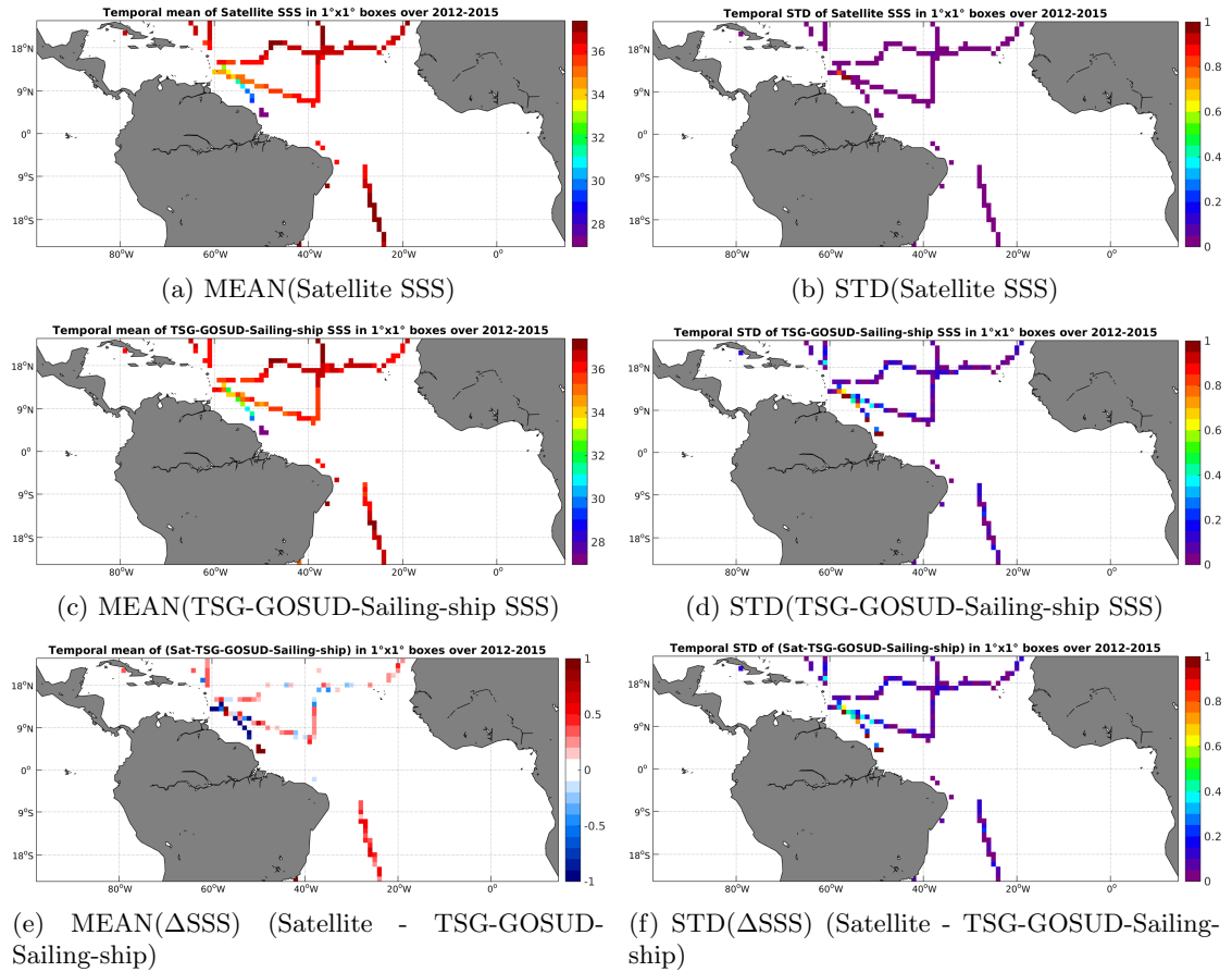
Figure 6: Temporal mean (left) and STD (right) of SSS from Aquarius-L3-JPL-V4-MONTHLY (top), TSG-GOSUD-Sailing-ship (middle), and of \Delta SSS (Satellite - TSG-GOSUD-Sailing-ship). Only match-up pairs are used to generate these maps.
