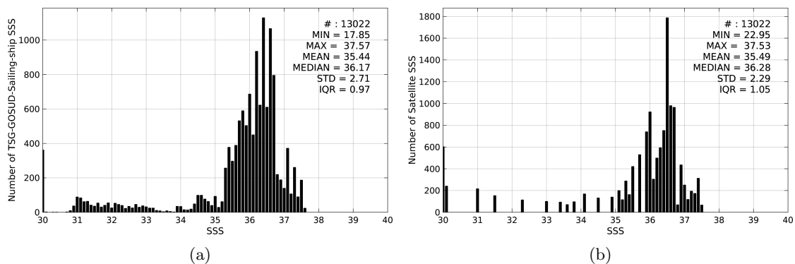
Figure 2: Histograms of SSS from TSG-GOSUD-Sailing-ship (a) and Aquarius-L3-JPL-V4-MONTHLY (b) considering all match-up pairs per bins of 0.1 over the Tropical Atlantic Ocean Pi-MEP region and for the full satellite product period.
