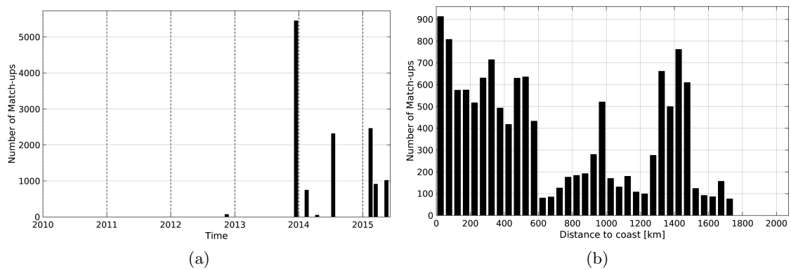
Figure 1: Number of match-ups between TSG-GOSUD-Sailing-ship and Aquarius-L3-JPL-V4-MONTHLY SSS as a function of time (a) and as function of the distance to coast (b) over the Tropical Atlantic Ocean Pi-MEP region and for the full satellite product period.
