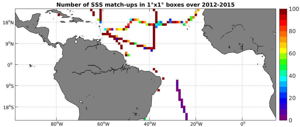
Figure 4: Number of SSS match-ups between TSG-GOSUD-Sailing-ship SSS and the Aquarius-L3-JPL-V4-MONTHLY SSS product for the Tropical Atlantic Ocean Pi-MEP region over 1^\circ \times 1^\circ boxes and for the full satellite product period.
