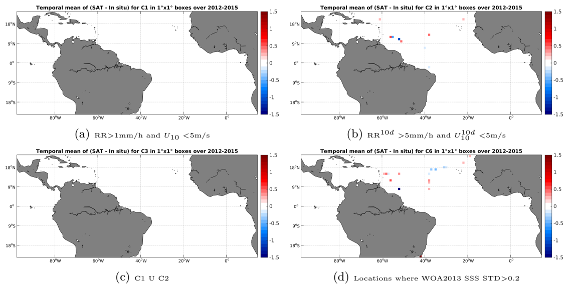
Figure 12: Temporal mean gridded over spatial boxes of size 1^\circ \times 1^\circ of \Delta SSS (Aquarius-L3-JPL-V4-MONTHLY - TSG-GOSUD-Sailing-ship) for 4 different subdatasets corresponding to:RR > 1 mm/h and U_{10} < 5 m/s (a), RR^{10d} > 5 mm/h and U_{10}^{10d} < 5 m/s (b), C1 U C2 (c),Locations where WOA2013 SSS STD > 0.2 (d).
