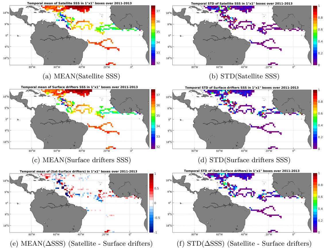
Figure 5: Temporal mean (left) and STD (right) of SSS from Aquarius-L3-JPL-V4-MONTHLY (top), Surface drifters (middle), and of \Delta SSS (Satellite - Surface drifters). Only match-up pairs are used to generate these maps.
