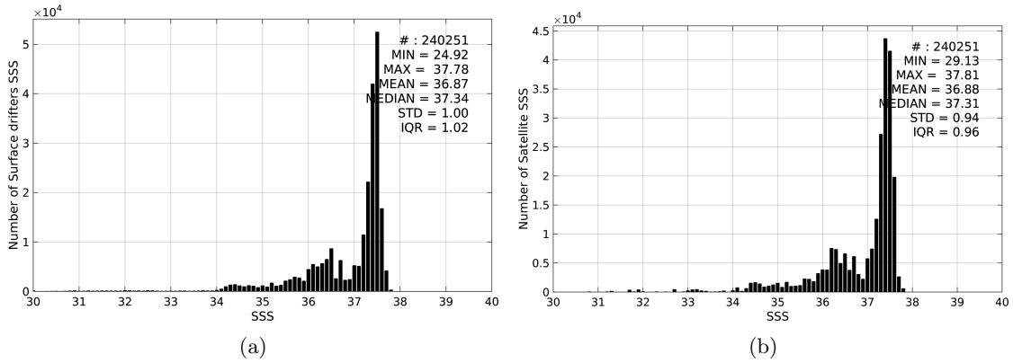
Figure 2: Histograms of SSS from Surface drifters (a) and Aquarius-L3-JPL-V4-MONTHLY (b) considering all match-up pairs per bins of 0.1 over the Tropical Atlantic Ocean Pi-MEP region and for the full satellite product period.
