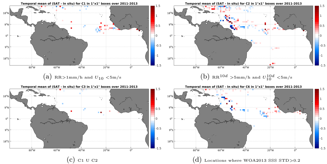
Figure 11: Temporal mean gridded over spatial boxes of size 1^\circ \times 1^\circ of \Delta SSS (Aquarius-L3-JPL-V4-MONTHLY - Surface drifters) for 4 different subdatasets corresponding to: RR > 1\text{mm/h} and U_{10} < 5\text{m/s} (a), RR^{10d} > 5\text{mm/h} and U_{10}^{10d} < 5\text{m/s} (b), C1 U C2 (c), Locations where WOA2013 SSS STD > 0.2 (d).
