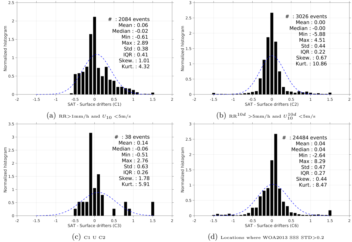
Figure 12: Normalized histogram of \Delta SSS (Aquarius-L3-JPL-V4-MONTHLY - Surface drifters) for 6 different subdatasets corresponding to: RR > 1\text{mm/h} and U_{10} < 5\text{m/s} (a), RR^{10d} > 5\text{mm/h} and U_{10}^{10d} < 5\text{m/s} (b), C1 U C2 (c), Locations where WOA2013 SSS STD > 0.2 (d).
