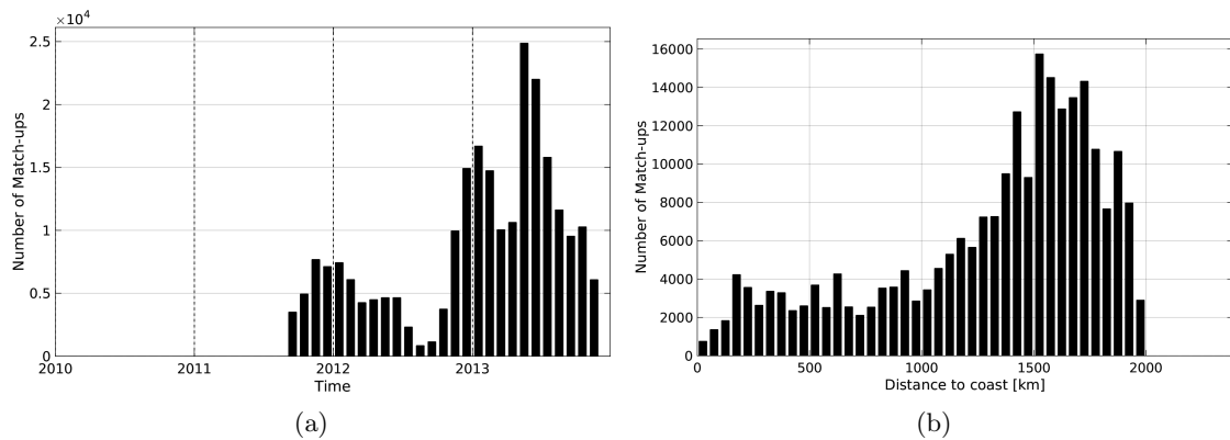
Figure 1: Number of match-ups between Surface drifters and Aquarius-L3-JPL-V4-MONTHLY SSS as a function of time (a) and as function of the distance to coast (b) over the Tropical Atlantic Ocean Pi-MEP region and for the full satellite product period.
