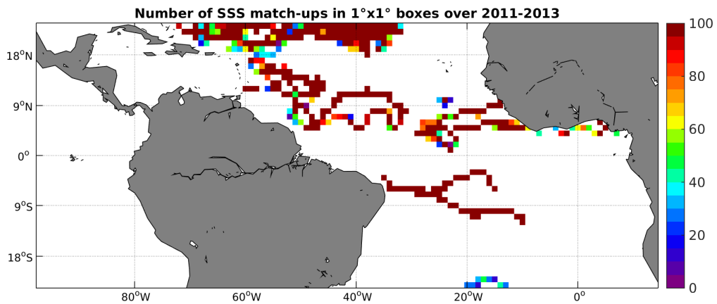
Figure 3: Number of SSS match-ups between Surface drifters SSS and the Aquarius-L3-JPL-V4-MONTHLY SSS product for the Tropical Atlantic Ocean Pi-MEP region over 1°x1° boxes and for the full satellite product period.
