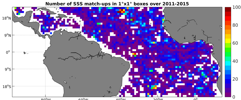
Figure 4: Number of SSS match-ups between Argo SSS and the Aquarius-L3-JPL-V4-MONTHLY SSS product for the Tropical Atlantic Ocean Pi-MEP region over 1^\circ \times 1^\circ boxes and for the full satellite product period.
