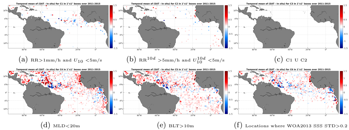
Figure 12: Temporal mean gridded over spatial boxes of size 1^\circ \times 1^\circ of \Delta SSS (Aquarius-L3-JPL-V4-MONTHLY - Argo) for 6 different subdatasets corresponding to: RR > 1 mm/h and U_{10} < 5 m/s (a), RR 10d > 5 mm/h and U_{10}^{10d} < 5 m/s (b), C1 U C2 (c), MLD < 20 m (d), BLT > 10 m (e), Locations where WOA2013 SSS STD > 0.2 (f).
