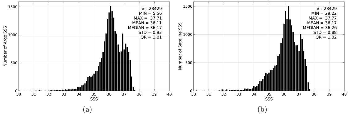
Figure 2: Histograms of SSS from Argo (a) and Aquarius-L3-JPL-V4-MONTHLY (b) considering all match-up pairs per bins of 0.1 over the Tropical Atlantic Ocean Pi-MEP region and for the full satellite product period.
