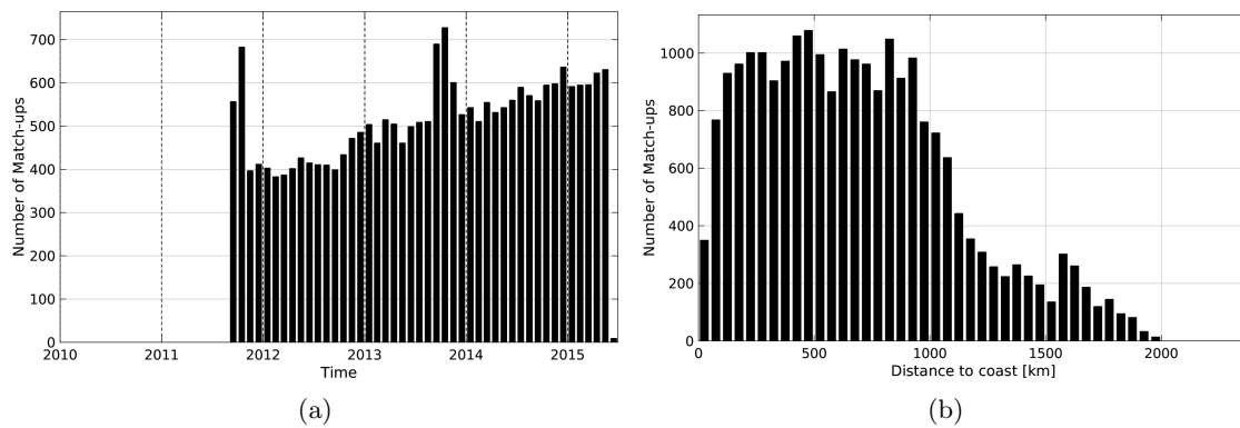
Figure 1: Number of match-ups between Argo and Aquarius-L3-JPL-V4-MONTHLY SSS as a function of time (a) and as function of the distance to coast (b) over the Tropical Atlantic Ocean Pi-MEP region and for the full satellite product period.
