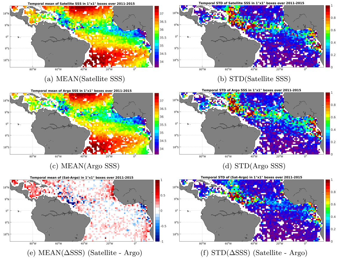
Figure 6: Temporal mean (left) and STD (right) of SSS from Aquarius-L3-JPL-V4-MONTHLY (top), Argo (middle), and of \Delta SSS (Satellite - Argo). Only match-up pairs are used to generate these maps.
