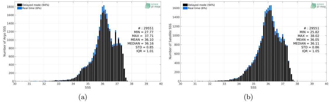
Figure 2: Histograms of SSS from Argo (a) and Aquarius SSS L2-AVERAGED OR v5 (NASA-GSFC) (b) considering all match-up pairs per bins of 0.1 over the Tropical Atlantic Ocean Pi-MEP region and for the full satellite product period.
