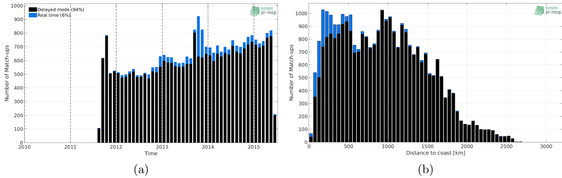
Figure 1: Number of match-ups between Argo and Aquarius SSS L2-AVERAGED OR v5 (NASA-GSFC) SSS as a function of time (a) and as function of the distance to coast (b) over the Tropical Atlantic Ocean Pi-MEP region and for the full satellite product period.
