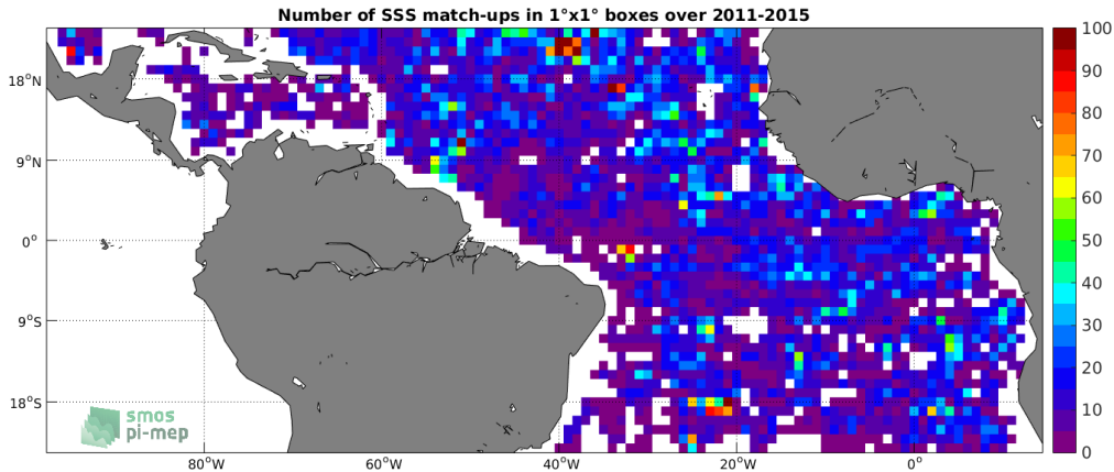
Figure 4: Number of SSS match-ups between Argo SSS and the Aquarius SSS L2-AVERAGED OR v5 (NASA-GSFC) SSS product for the Tropical Atlantic Ocean Pi-MEP region over 1^\circ \times 1^\circ boxes and for the full satellite product period.
