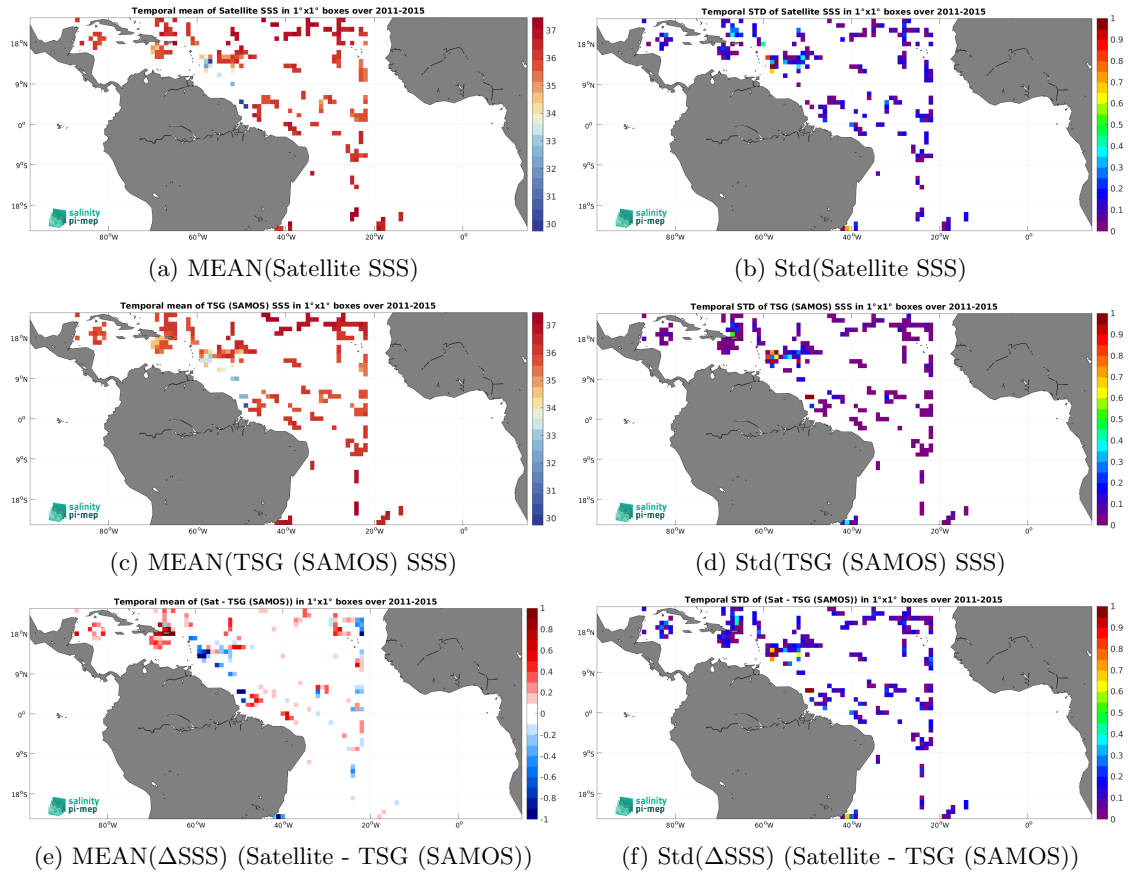
Figure 7: Temporal mean (left) and Std (right) of SSS from Aquarius SSS L2 OR v5 (NASA-GSFC) (top), TSG (SAMOS) (middle), and of \Delta SSS (Satellite - TSG (SAMOS)). Only match-up pairs are used to generate these maps.
