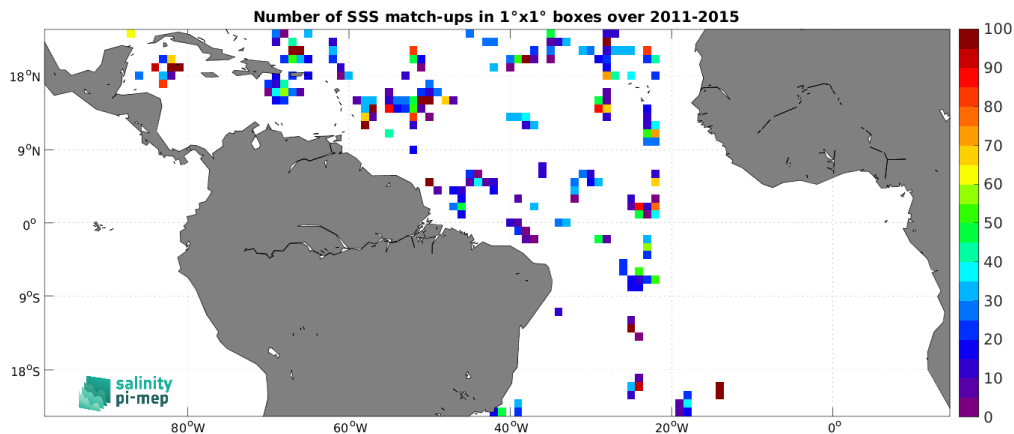
Figure 5: Number of SSS match-ups between TSG (SAMOS) SSS and the Aquarius SSS L2 OR v5 (NASA-GSFC) SSS product for the Tropical Atlantic Ocean Pi-MEP region over 1^\circ \times 1^\circ boxes and for the full satellite product period.
