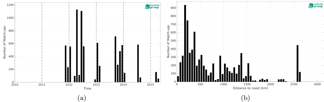
Figure 2: Number of match-ups between TSG (SAMOS) and Aquarius SSS L2 OR v5 (NASA-GSFC) SSS as a function of time (a) and as function of the distance to coast (b) over the Tropical Atlantic Ocean Pi-MEP region and for the full satellite product period.
