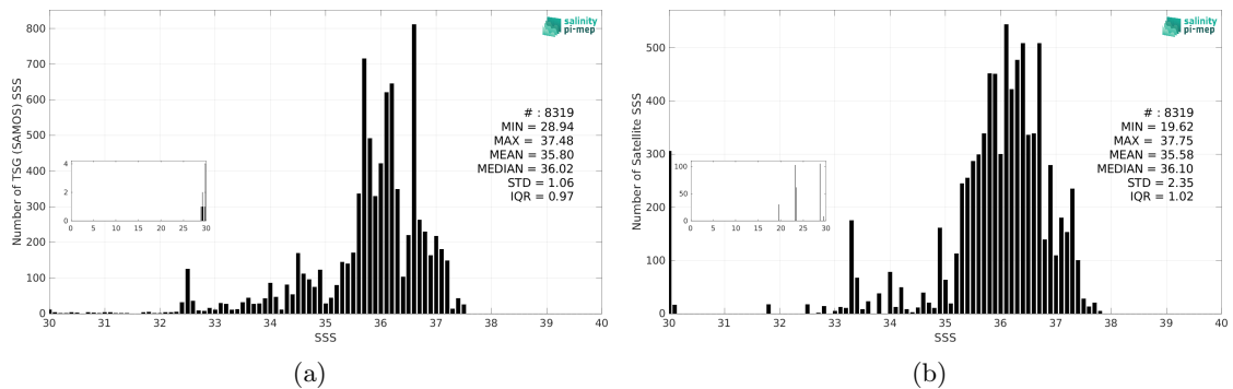
Figure 3: Histograms of SSS from TSG (SAMOS) (a) and Aquarius SSS L2 OR v5 (NASA-GSFC) (b) considering all match-up pairs per bins of 0.1 over the Tropical Atlantic Ocean Pi-MEP region and for the full satellite product period.
