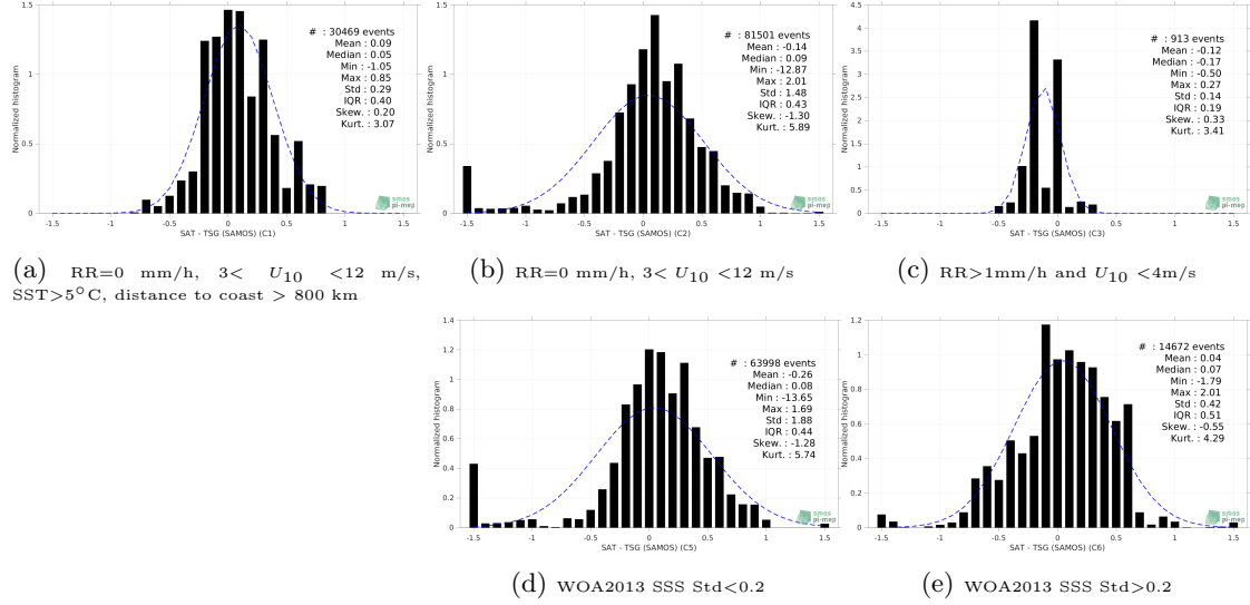
Figure 13: Normalized histogram of \Delta SSS (Aquarius SSS L2 OR v5 (NASA-GSFC) - TSG (SAMOS)) for 5 different subdatasets corresponding to: RR=0 mm/h, 3 < U_{10} < 12 m/s, SST>5°C, distance to coast > 800 km (a), RR=0 mm/h, 3 < U_{10} < 12 m/s (b), RR>1mm/h and U_{10} < 4 m/s (c), WOA2013 SSS Std<0.2 (d), WOA2013 SSS Std>0.2 (e).
