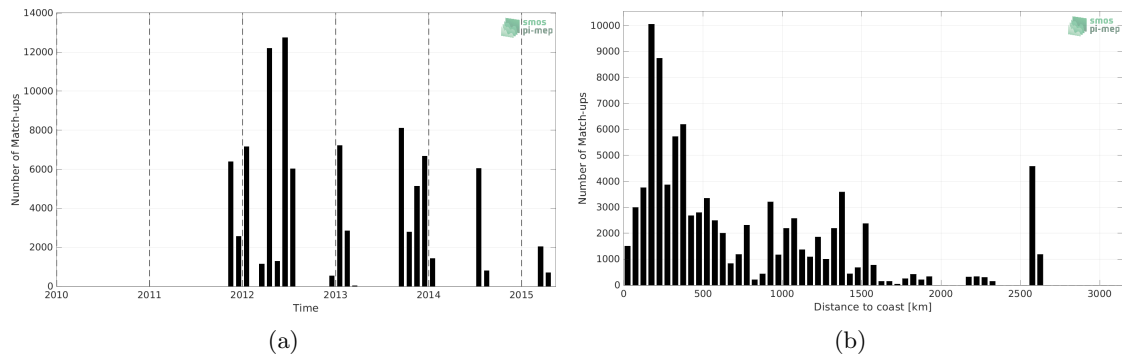
Figure 1: Number of match-ups between TSG (SAMOS) and Aquarius SSS L2 OR v5 (NASA-GSFC) SSS as a function of time (a) and as function of the distance to coast (b) over the Tropical Atlantic Ocean Pi-MEP region and for the full satellite product period.
