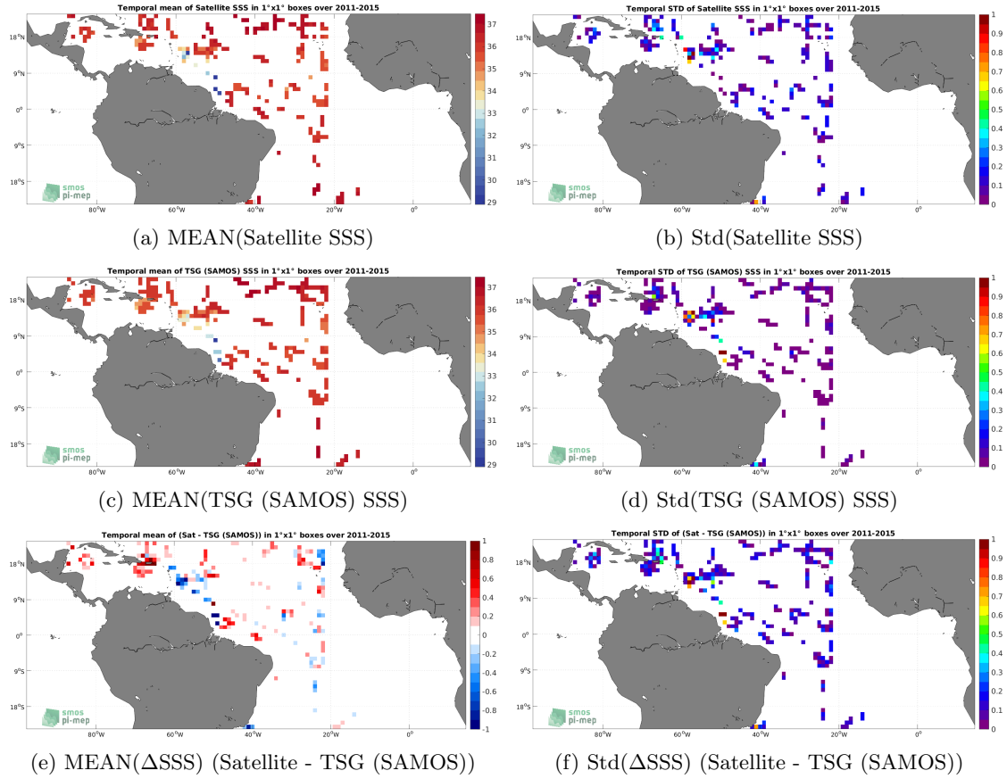
Figure 6: Temporal mean (left) and Std (right) of SSS from Aquarius SSS L2 OR v5 (NASA-GSFC) (top), TSG (SAMOS) (middle), and of \Delta SSS (Satellite - TSG (SAMOS)). Only match-up pairs are used to generate these maps.
