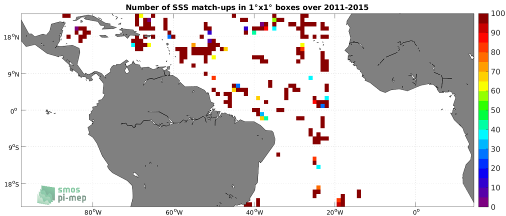
Figure 4: Number of SSS match-ups between TSG (SAMOS) SSS and the Aquarius SSS L2 OR v5 (NASA-GSFC) SSS product for the Tropical Atlantic Ocean Pi-MEP region over 1^\circ \times 1^\circ boxes and for the full satellite product period.
