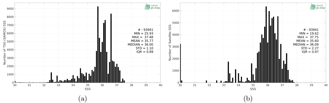
Figure 2: Histograms of SSS from TSG (SAMOS) (a) and Aquarius SSS L2 OR v5 (NASA-GSFC) (b) considering all match-up pairs per bins of 0.1 over the Tropical Atlantic Ocean Pi-MEP region and for the full satellite product period.
