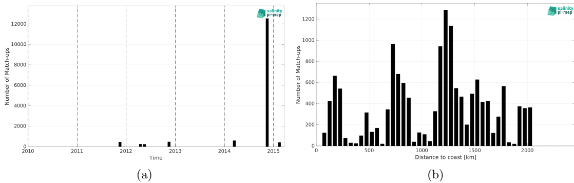
Figure 2: Number of match-ups between TSG (Polarstern) and Aquarius SSS L2 OR v5 (NASA-GSFC) SSS as a function of time (a) and as function of the distance to coast (b) over the Tropical Atlantic Ocean Pi-MEP region and for the full satellite product period.
