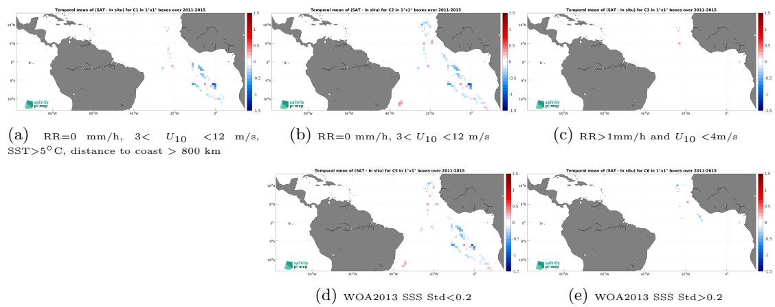
Figure 14: Temporal mean gridded over spatial boxes of size 1^\circ \times 1^\circ of \Delta SSS (Aquarius SSS L2 OR v5 (NASA-GSFC) - TSG (Polarstern)) for 5 different subdatasets corresponding to:RR=0 mm/h, 3 < U_{10} < 12 m/s, SST >5^\circ\text{C} , distance to coast > 800 km (a), RR=0 mm/h, 3 < U_{10} < 12 m/s (b), RR >1 mm/h and U_{10} < 4 m/s (c), WOA2013 SSS Std <0.2 (d), WOA2013 SSS Std >0.2 (e).
