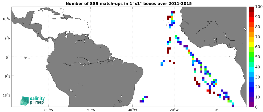
Figure 5: Number of SSS match-ups between TSG (Polarstern) SSS and the Aquarius SSS L2 OR v5 (NASA-GSFC) SSS product for the Tropical Atlantic Ocean Pi-MEP region over 1^\circ \times 1^\circ boxes and for the full satellite product period.
