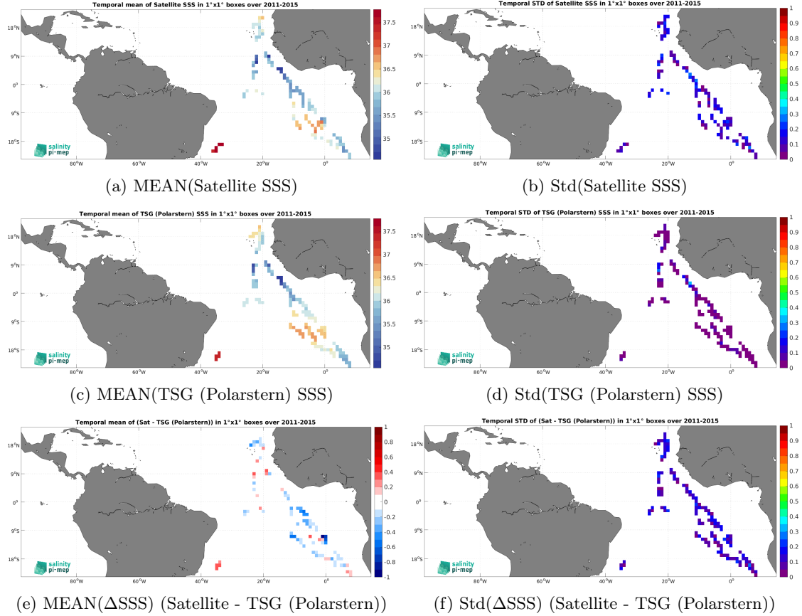
Figure 7: Temporal mean (left) and Std (right) of SSS from Aquarius SSS L2 OR v5 (NASA-GSFC) (top), TSG (Polarstern) (middle), and of \Delta\text{SSS} (Satellite - TSG (Polarstern)). Only match-up pairs are used to generate these maps.
