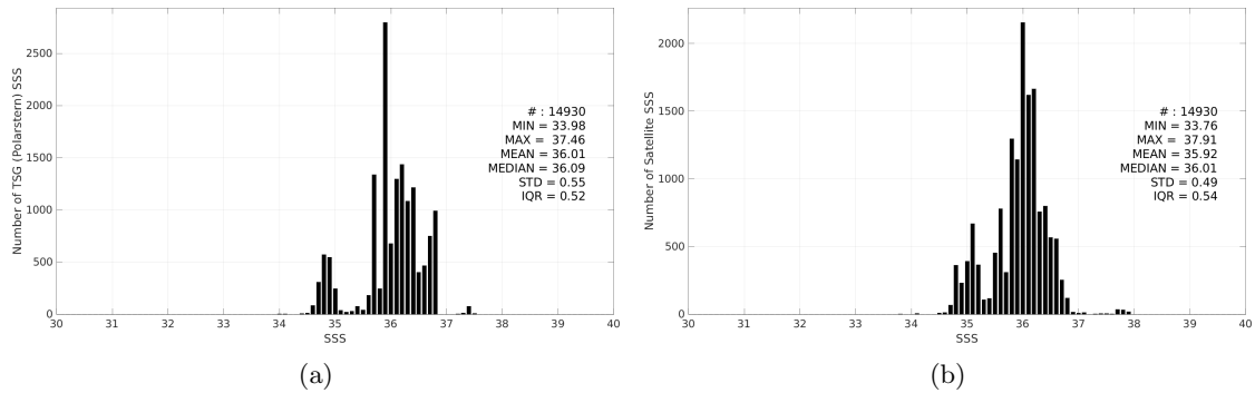
Figure 3: Histograms of SSS from TSG (Polarstern) (a) and Aquarius SSS L2 OR v5 (NASA-GSFC) (b) considering all match-up pairs per bins of 0.1 over the Tropical Atlantic Ocean Pi-MEP region and for the full satellite product period.
