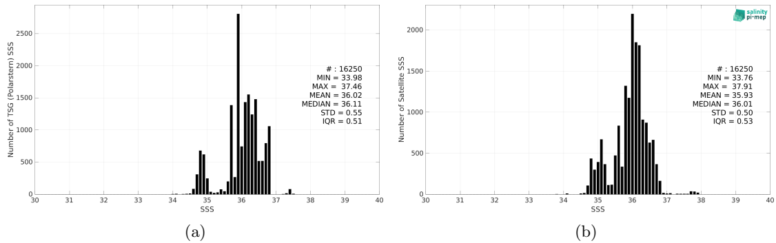
Figure 2: Histograms of SSS from TSG (Polarstern) (a) and Aquarius SSS L2 OR v5 (NASA-GSFC) (b) considering all match-up pairs per bins of 0.1 over the Tropical Atlantic Ocean Pi-MEP region and for the full satellite product period.
