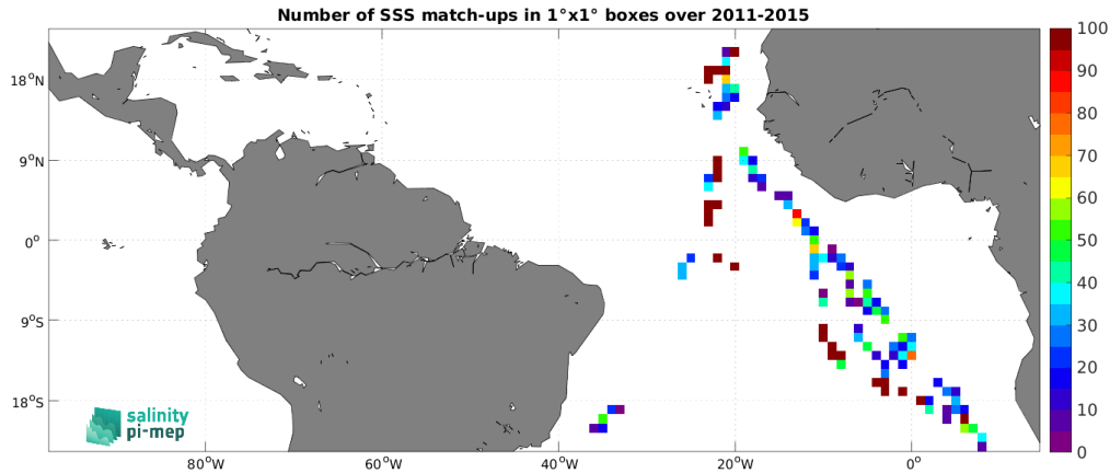
Figure 4: Number of SSS match-ups between TSG (Polarstern) SSS and the Aquarius SSS L2 OR v5 (NASA-GSFC) SSS product for the Tropical Atlantic Ocean Pi-MEP region over 1^\circ \times 1^\circ boxes and for the full satellite product period.
