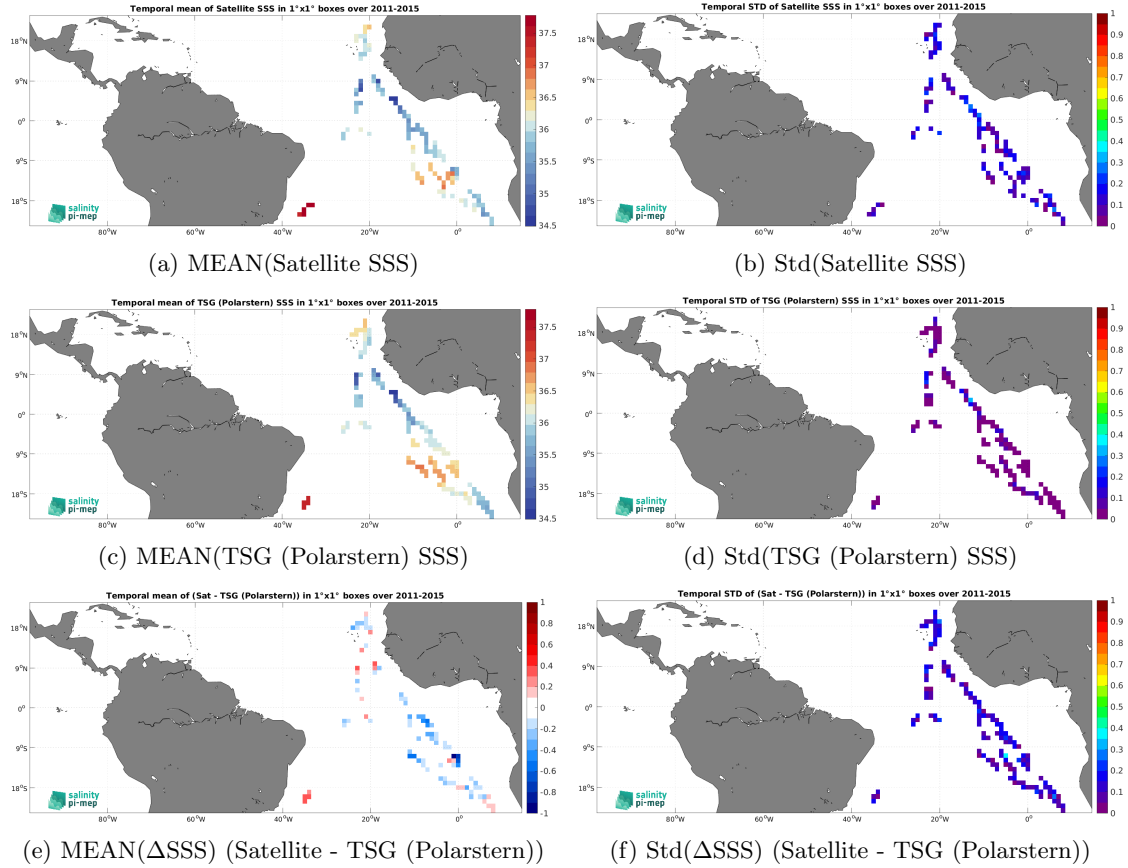
Figure 6: Temporal mean (left) and Std (right) of SSS from Aquarius SSS L2 OR v5 (NASA-GSFC) (top), TSG (Polarstern) (middle), and of \Delta\text{SSS} (Satellite - TSG (Polarstern)). Only match-up pairs are used to generate these maps.
