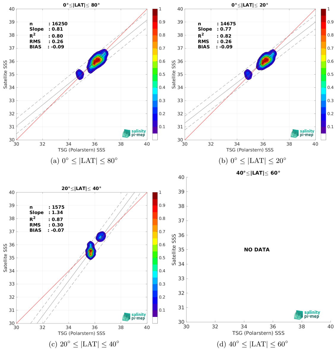
Figure 9: Contour maps of the concentration of Aquarius SSS L2 OR v5 (NASA-GSFC) SSS (y-axis) versus TSG (Polarstern) SSS (x-axis) at match-up pairs for different latitude bands. For each plot, the red line shows x=y . The black thin and dashed lines indicate a linear fit through the data cloud and the \pm 95\% confidence levels, respectively. The number match-up pairs n , the slope and R^2 coefficient of the linear fit, the root mean square (RMS) and the mean bias between satellite and in situ data are indicated for each latitude band in each plots.
