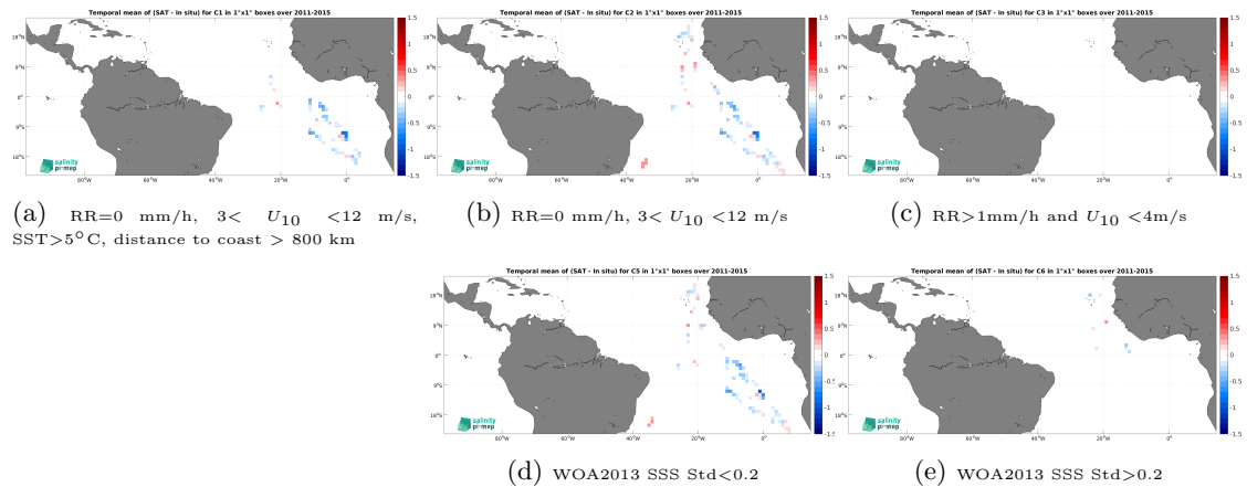
Figure 12: Temporal mean gridded over spatial boxes of size 1^\circ \times 1^\circ of \Delta SSS (Aquarius SSS L2 OR v5 (NASA-GSFC) - TSG (Polarstern)) for 5 different subdatasets corresponding to:RR=0 mm/h, 3 < U_{10} < 12 m/s, SST >5^\circ\text{C} , distance to coast > 800 km (a), RR=0 mm/h, 3 < U_{10} < 12 m/s (b), RR >1 mm/h and U_{10} < 4 m/s (c), WOA2013 SSS Std <0.2 (d), WOA2013 SSS Std >0.2 (e).
