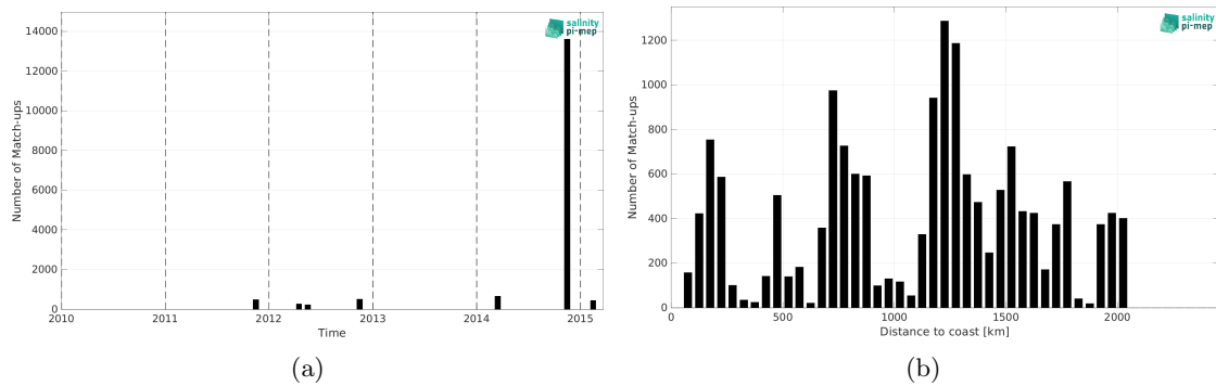
Figure 1: Number of match-ups between TSG (Polarstern) and Aquarius SSS L2 OR v5 (NASA-GSFC) SSS as a function of time (a) and as function of the distance to coast (b) over the Tropical Atlantic Ocean Pi-MEP region and for the full satellite product period.
