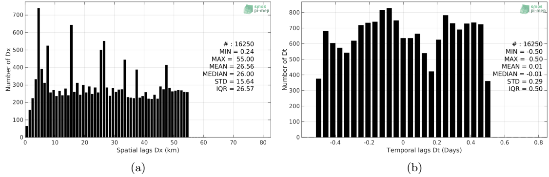
Figure 5: Histograms of the spatial (a) and temporal (b) lags between the time of the TSG-POLARSTERN measurements and the date of the corresponding Aquarius-L2-OR-V5 SSS product.
