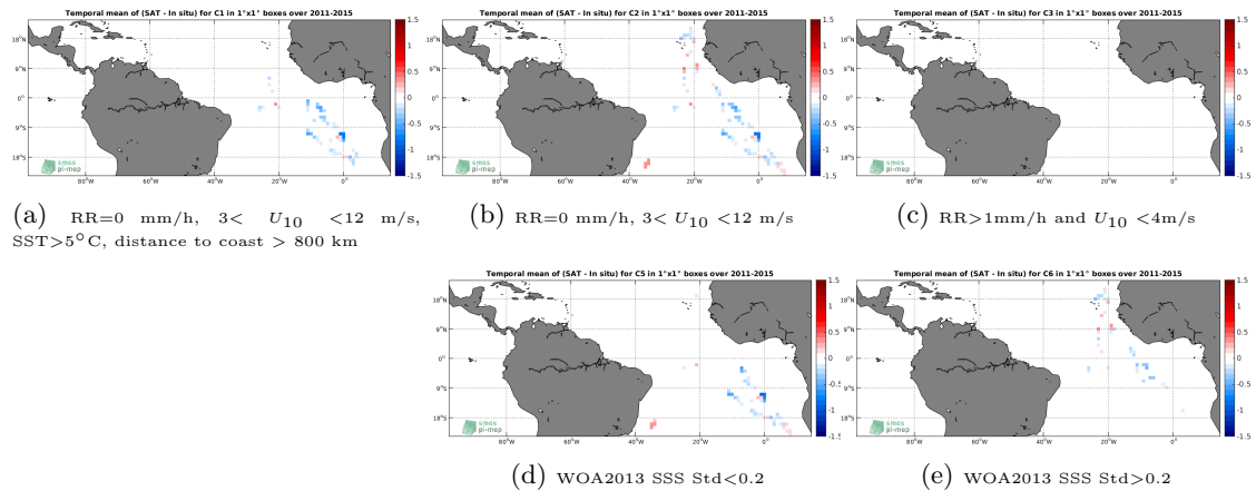
Figure 12: Temporal mean gridded over spatial boxes of size 1^\circ \times 1^\circ of \Delta SSS (Aquarius-L2-OR-V5 - TSG-POLARSTERN) for 5 different subdatasets corresponding to:RR=0 mm/h, 3 < U_{10} < 12 m/s, SST >5^\circ\text{C} , distance to coast > 800 km (a), RR=0 mm/h, 3 < U_{10} < 12 m/s (b), RR >1 mm/h and U_{10} < 4 m/s (c), WOA2013 SSS Std <0.2 (d), WOA2013 SSS Std >0.2 (e).
