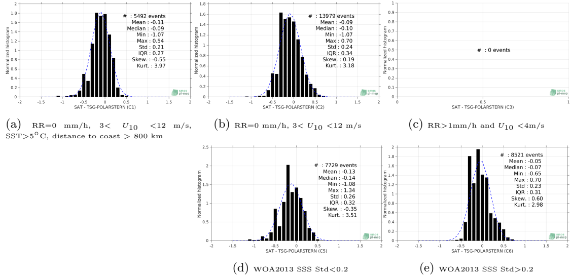
Figure 13: Normalized histogram of \Delta SSS (Aquarius-L2-OR-V5 - TSG-POLARSTERN) for 5 different subdatasets corresponding to: RR=0 mm/h, 3 < U_{10} < 12 m/s, SST > 5°C, distance to coast > 800 km (a), RR=0 mm/h, 3 < U_{10} < 12 m/s (b), RR > 1mm/h and U_{10} < 4 m/s (c), WOA2013 SSS Std < 0.2 (d), WOA2013 SSS Std > 0.2 (e).
