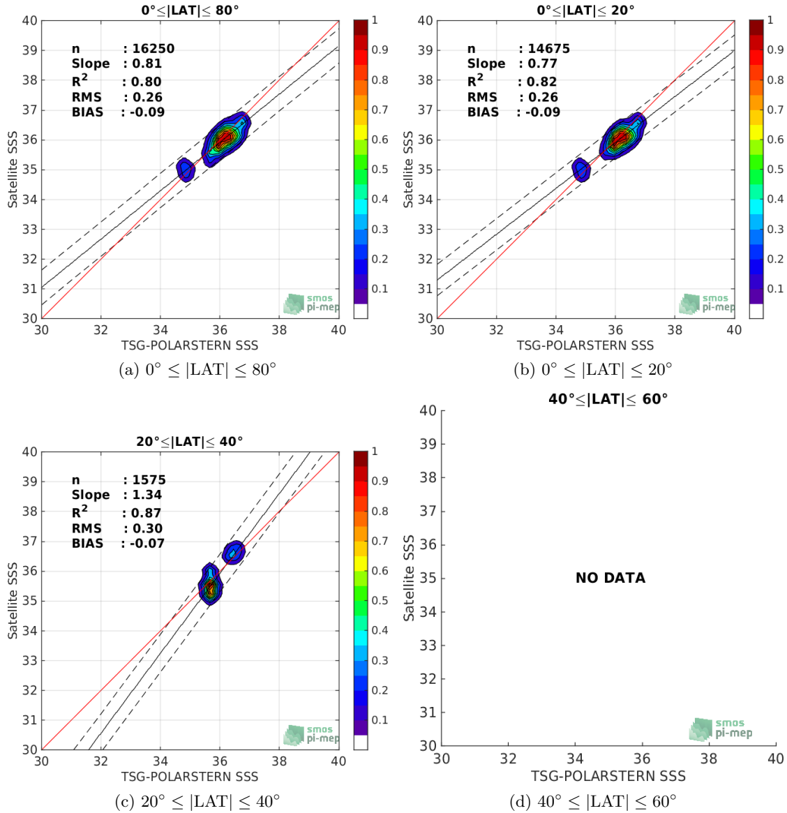
Figure 9: Contour maps of the concentration of Aquarius-L2-OR-V5 SSS (y-axis) versus TSG-POLARSTERN SSS (x-axis) at match-up pairs for different latitude bands. For each plot, the red line shows x=y . The black thin and dashed lines indicate a linear fit through the data cloud and the \pm 95\% confidence levels, respectively. The number match-up pairs n , the slope and R^2 coefficient of the linear fit, the root mean square (RMS) and the mean bias between satellite and in situ data are indicated for each latitude band in each plots.
