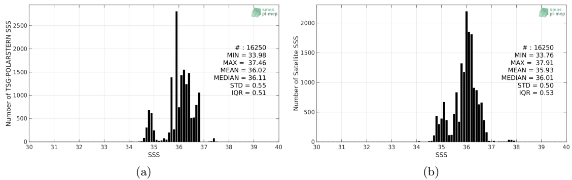
Figure 2: Histograms of SSS from TSG-POLARSTERN (a) and Aquarius-L2-OR-V5 (b) considering all match-up pairs per bins of 0.1 over the Tropical Atlantic Ocean Pi-MEP region and for the full satellite product period.
