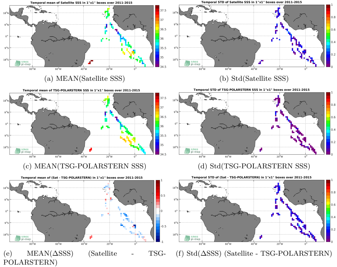
Figure 6: Temporal mean (left) and Std (right) of SSS from Aquarius-L2-OR-V5 (top), TSG-POLARSTERN (middle), and of \Delta SSS (Satellite - TSG-POLARSTERN). Only match-up pairs are used to generate these maps.
