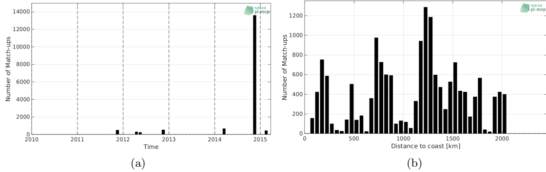
Figure 1: Number of match-ups between TSG-POLARSTERN and Aquarius-L2-OR-V5 SSS as a function of time (a) and as function of the distance to coast (b) over the Tropical Atlantic Ocean Pi-MEP region and for the full satellite product period.
