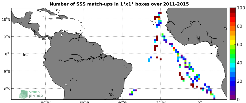
Figure 4: Number of SSS match-ups between TSG-POLARSTERN SSS and the Aquarius-L2-OR-V5 SSS product for the Tropical Atlantic Ocean Pi-MEP region over 1^\circ \times 1^\circ boxes and for the full satellite product period.
