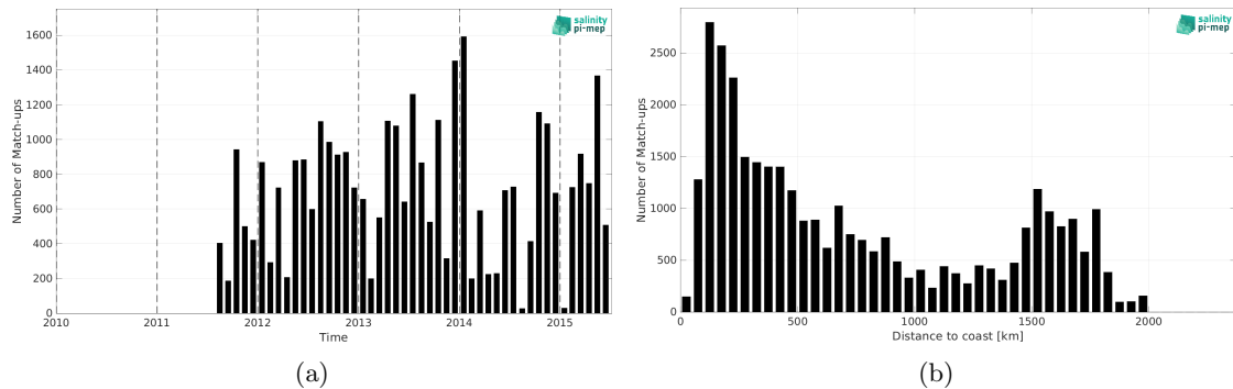
Figure 2: Number of match-ups between TSG (LEGOS-DM) and Aquarius SSS L2 OR v5 (NASA-GSFC) SSS as a function of time (a) and as function of the distance to coast (b) over the Tropical Atlantic Ocean Pi-MEP region and for the full satellite product period.
