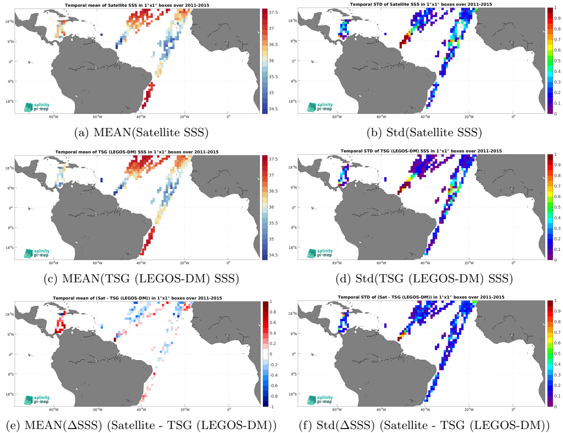
Figure 7: Temporal mean (left) and Std (right) of SSS from Aquarius SSS L2 OR v5 (NASA-GSFC) (top), TSG (LEGOS-DM) (middle), and of \Delta SSS (Satellite - TSG (LEGOS-DM)). Only match-up pairs are used to generate these maps.
