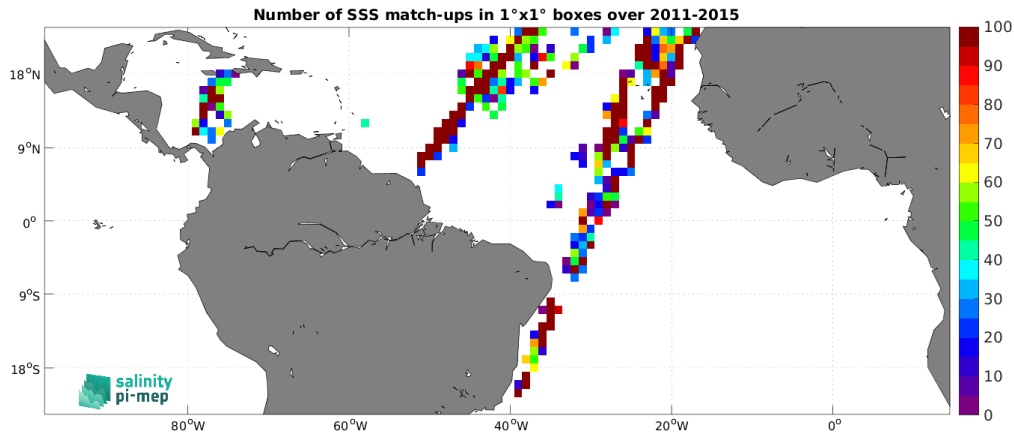
Figure 5: Number of SSS match-ups between TSG (LEGOS-DM) SSS and the Aquarius SSS L2 OR v5 (NASA-GSFC) SSS product for the Tropical Atlantic Ocean Pi-MEP region over 1^\circ \times 1^\circ boxes and for the full satellite product period.
