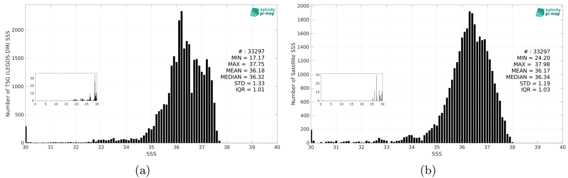
Figure 3: Histograms of SSS from TSG (LEGOS-DM) (a) and Aquarius SSS L2 OR v5 (NASA-GSFC) (b) considering all match-up pairs per bins of 0.1 over the Tropical Atlantic Ocean Pi-MEP region and for the full satellite product period.
