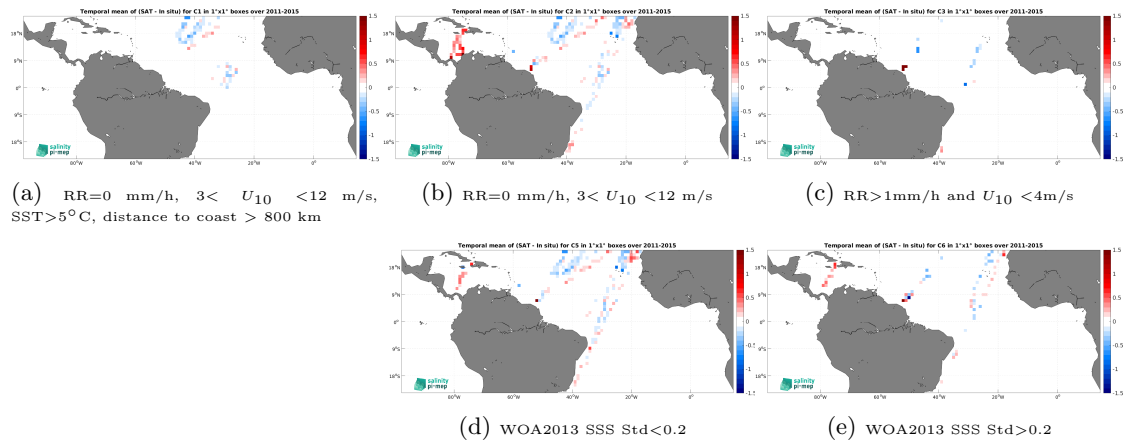
Figure 12: Temporal mean gridded over spatial boxes of size 1^\circ \times 1^\circ of \Delta\text{SSS} (Aquarius SSS L2 OR v5 (NASA-GSFC) - TSG (LEGOS-DM)) for 5 different subdatasets corresponding to:RR=0 mm/h, 3 < U_{10} < 12 m/s, SST >5^\circ\text{C} , distance to coast > 800 km (a), RR=0 mm/h, 3 < U_{10} < 12 m/s (b), RR >1 mm/h and U_{10} < 4 m/s (c), WOA2013 SSS Std <0.2 (d), WOA2013 SSS Std >0.2 (e).
