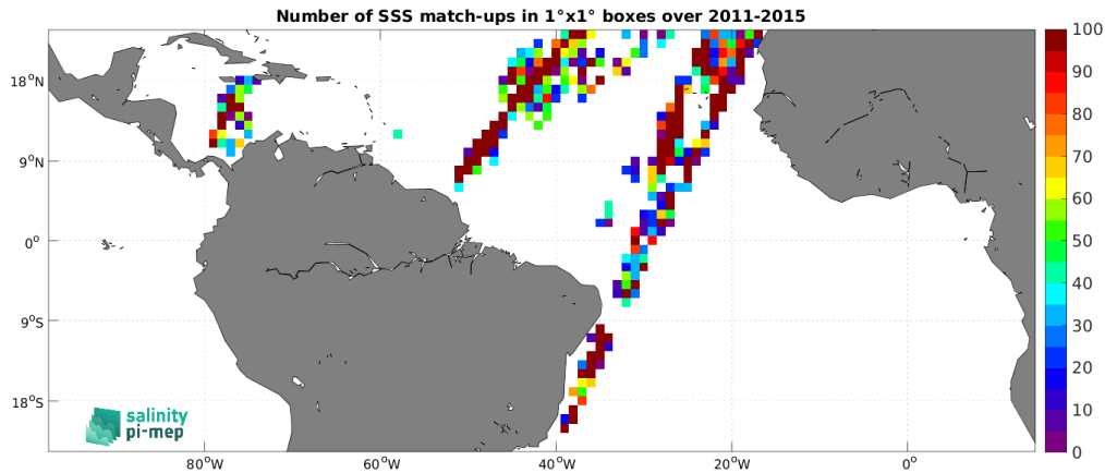
Figure 4: Number of SSS match-ups between TSG (LEGOS-DM) SSS and the Aquarius SSS L2 OR v5 (NASA-GSFC) SSS product for the Tropical Atlantic Ocean Pi-MEP region over 1^\circ \times 1^\circ boxes and for the full satellite product period.
