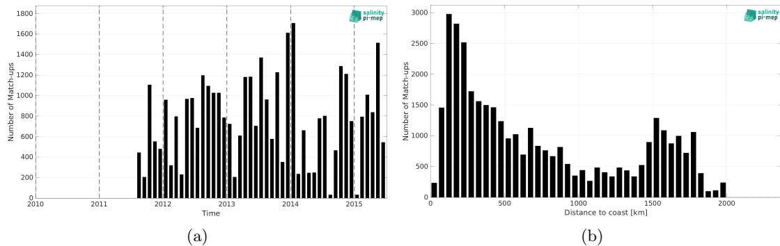
Figure 1: Number of match-ups between TSG (LEGOS-DM) and Aquarius SSS L2 OR v5 (NASA-GSFC) SSS as a function of time (a) and as function of the distance to coast (b) over the Tropical Atlantic Ocean Pi-MEP region and for the full satellite product period.
