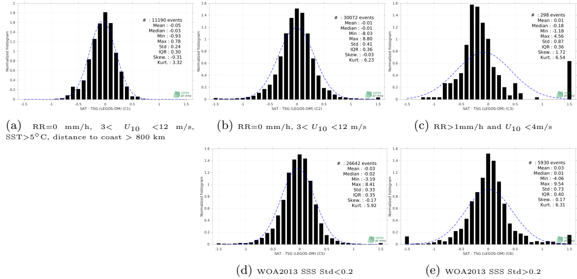
Figure 13: Normalized histogram of \Delta\text{SSS} (Aquarius SSS L2 OR v5 (NASA-GSFC) - TSG (LEGOS-DM)) for 5 different subdatasets corresponding to: RR=0 mm/h, 3 < U_{10} < 12 m/s, SST>5°C, distance to coast > 800 km (a), RR=0 mm/h, 3 < U_{10} < 12 m/s (b), RR>1mm/h and U_{10} < 4 m/s (c), WOA2013 SSS Std<0.2 (d), WOA2013 SSS Std>0.2 (e).
