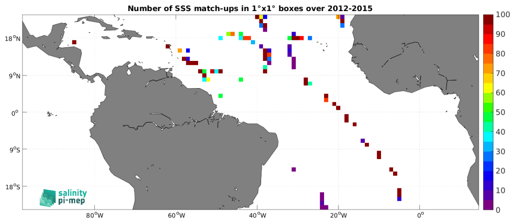
Figure 5: Number of SSS match-ups between TSG (GOSUD-Sailing-ship) SSS and the Aquarius SSS L2 OR v5 (NASA-GSFC) SSS product for the Tropical Atlantic Ocean Pi-MEP region over 1^\circ \times 1^\circ boxes and for the full satellite product period.
