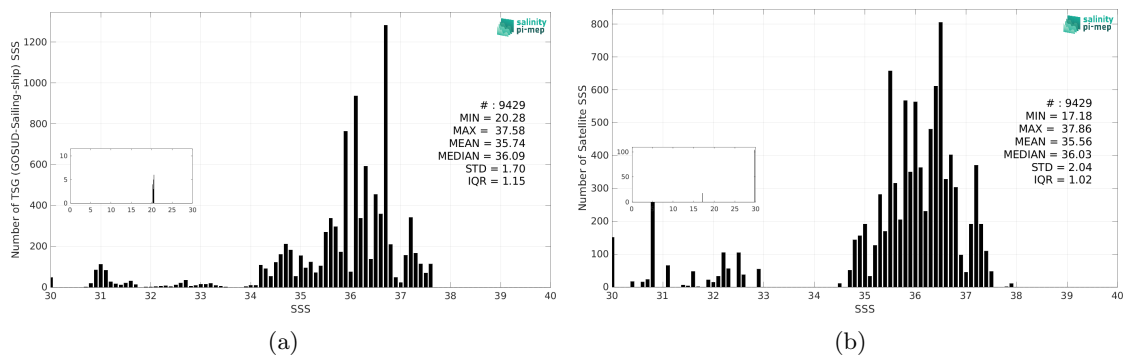
Figure 3: Histograms of SSS from TSG (GOSUD-Sailing-ship) (a) and Aquarius SSS L2 OR v5 (NASA-GSFC) (b) considering all match-up pairs per bins of 0.1 over the Tropical Atlantic Ocean Pi-MEP region and for the full satellite product period.
