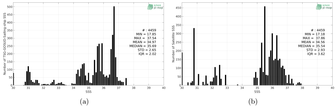
Figure 2: Histograms of SSS from TSG-GOSUD-Sailing-ship (a) and Aquarius-L2-OR-V5 (b) considering all match-up pairs per bins of 0.1 over the Tropical Atlantic Ocean Pi-MEP region and for the full satellite product period.
