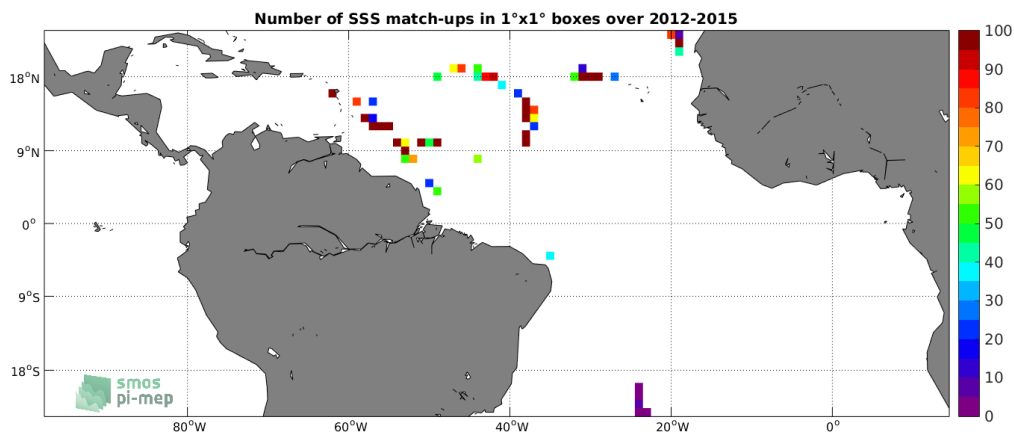
Figure 4: Number of SSS match-ups between TSG-GOSUD-Sailing-ship SSS and the Aquarius-L2-OR-V5 SSS product for the Tropical Atlantic Ocean Pi-MEP region over 1^\circ \times 1^\circ boxes and for the full satellite product period.
