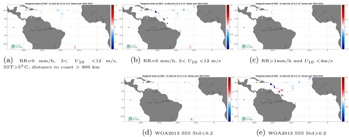
Figure 12: Temporal mean gridded over spatial boxes of size 1^\circ \times 1^\circ of \Delta SSS (Aquarius-L2-OR-V5 - TSG-GOSUD-Sailing-ship) for 5 different subdatasets corresponding to:RR=0 mm/h, 3 < U_{10} < 12 m/s, SST >5^\circ\text{C} , distance to coast > 800 km (a), RR=0 mm/h, 3 < U_{10} < 12 m/s (b), RR >1 mm/h and U_{10} < 4 m/s (c), WOA2013 SSS Std <0.2 (d), WOA2013 SSS Std >0.2 (e).
