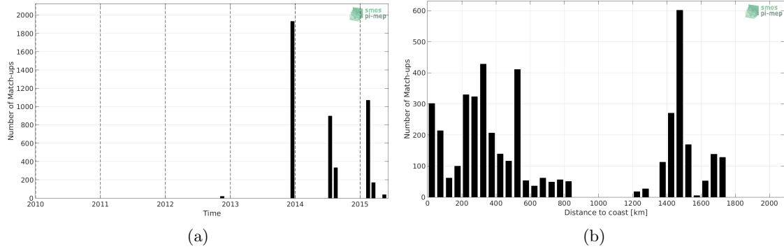
Figure 1: Number of match-ups between TSG-GOSUD-Sailing-ship and Aquarius-L2-OR-V5 SSS as a function of time (a) and as function of the distance to coast (b) over the Tropical Atlantic Ocean Pi-MEP region and for the full satellite product period.
