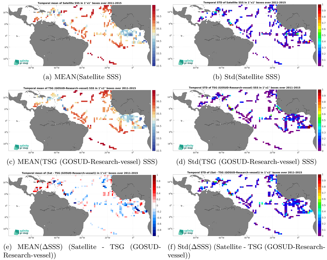
Figure 7: Temporal mean (left) and Std (right) of SSS from Aquarius SSS L2 OR v5 (NASA-GSFC) (top), TSG (GOSUD-Research-vessel) (middle), and of \Delta SSS (Satellite - TSG (GOSUD-Research-vessel)). Only match-up pairs are used to generate these maps.
