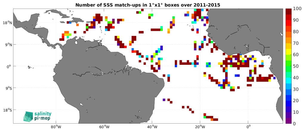
Figure 5: Number of SSS match-ups between TSG (GOSUD-Research-vessel) SSS and the Aquarius SSS L2 OR v5 (NASA-GSFC) SSS product for the Tropical Atlantic Ocean Pi-MEP region over 1^\circ \times 1^\circ boxes and for the full satellite product period.
