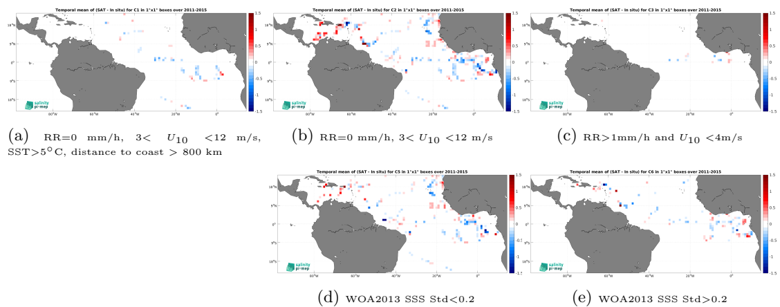
Figure 14: Temporal mean gridded over spatial boxes of size 1^\circ \times 1^\circ of \Delta SSS (Aquarius SSS L2 OR v5 (NASA-GSFC) - TSG (GOSUD-Research-vessel)) for 5 different subdatasets corresponding to:RR=0 mm/h, 3 < U_{10} < 12 m/s, SST >5^\circ\text{C} , distance to coast > 800 km (a), RR=0 mm/h, 3 < U_{10} < 12 m/s (b), RR >1 mm/h and U_{10} < 4 m/s (c), WOA2013 SSS Std <0.2 (d), WOA2013 SSS Std >0.2 (e).
