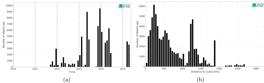
Figure 2: Number of match-ups between TSG (GOSUD-Research-vessel) and Aquarius SSS L2 OR v5 (NASA-GSFC) SSS as a function of time (a) and as function of the distance to coast (b) over the Tropical Atlantic Ocean Pi-MEP region and for the full satellite product period.
