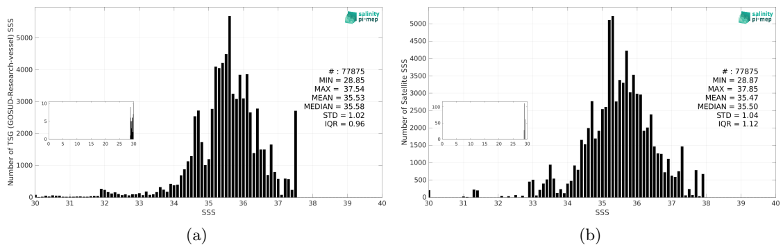
Figure 3: Histograms of SSS from TSG (GOSUD-Research-vessel) (a) and Aquarius SSS L2 OR v5 (NASA-GSFC) (b) considering all match-up pairs per bins of 0.1 over the Tropical Atlantic Ocean Pi-MEP region and for the full satellite product period.
