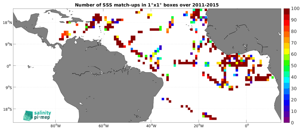
Figure 4: Number of SSS match-ups between TSG (GOSUD-Research-vessel) SSS and the Aquarius SSS L2 OR v5 (NASA-GSFC) SSS product for the Tropical Atlantic Ocean Pi-MEP region over 1^\circ \times 1^\circ boxes and for the full satellite product period.
