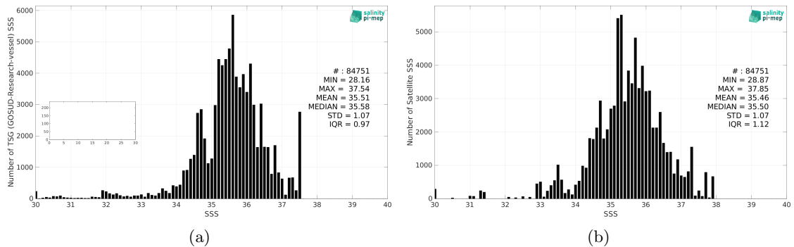
Figure 2: Histograms of SSS from TSG (GOSUD-Research-vessel) (a) and Aquarius SSS L2 OR v5 (NASA-GSFC) (b) considering all match-up pairs per bins of 0.1 over the Tropical Atlantic Ocean Pi-MEP region and for the full satellite product period.
