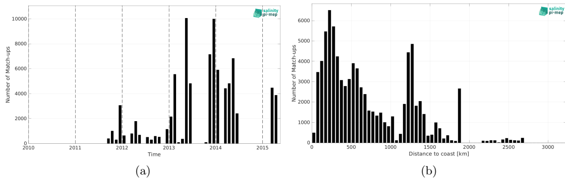
Figure 1: Number of match-ups between TSG (GOSUD-Research-vessel) and Aquarius SSS L2 OR v5 (NASA-GSFC) SSS as a function of time (a) and as function of the distance to coast (b) over the Tropical Atlantic Ocean Pi-MEP region and for the full satellite product period.
