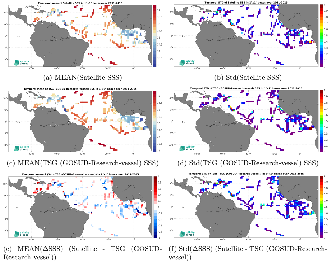
Figure 6: Temporal mean (left) and Std (right) of SSS from Aquarius SSS L2 OR v5 (NASA-GSFC) (top), TSG (GOSUD-Research-vessel) (middle), and of \Delta SSS (Satellite - TSG (GOSUD-Research-vessel)). Only match-up pairs are used to generate these maps.
