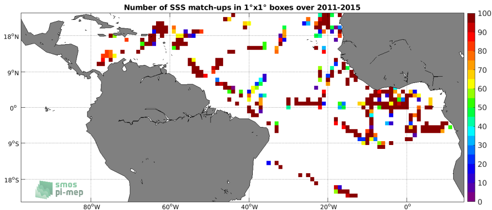
Figure 4: Number of SSS match-ups between TSG (GOSUD-Research-vessel) SSS and the Aquarius SSS L2 OR v5 (NASA-GSFC) SSS product for the Tropical Atlantic Ocean Pi-MEP region over 1°x1° boxes and for the full satellite product period.
