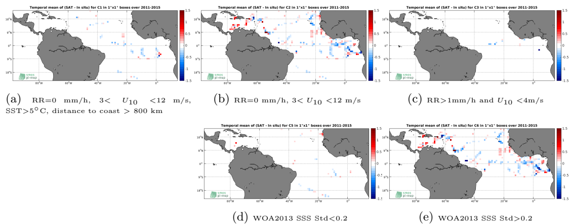
Figure 12: Temporal mean gridded over spatial boxes of size 1^\circ \times 1^\circ of \Delta\text{SSS} (Aquarius-L2-OR-V5 - TSG-GOSUD-Research-vessel) for 5 different subdatasets corresponding to:RR=0 mm/h, 3 < U_{10} < 12 m/s, SST>5°C, distance to coast > 800 km (a), RR=0 mm/h, 3 < U_{10} < 12 m/s (b), RR>1mm/h and U_{10} < 4 m/s (c), WOA2013 SSS Std<0.2 (d), WOA2013 SSS Std>0.2 (e).
