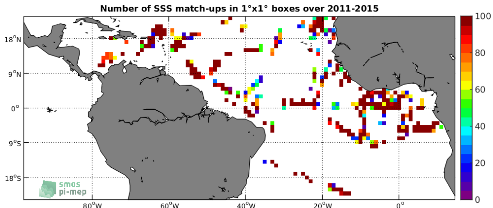
Figure 4: Number of SSS match-ups between TSG-GOSUD-Research-vessel SSS and the Aquarius-L2-OR-V5 SSS product for the Tropical Atlantic Ocean Pi-MEP region over 1°x1° boxes and for the full satellite product period.
