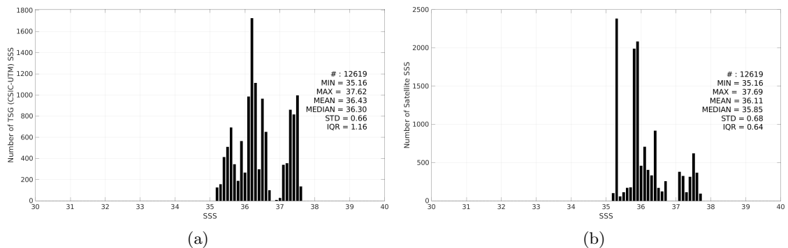
Figure 3: Histograms of SSS from TSG (CSIC-UTM) (a) and Aquarius SSS L2 OR v5 (NASA-GSFC) (b) considering all match-up pairs per bins of 0.1 over the Tropical Atlantic Ocean Pi-MEP region and for the full satellite product period.
