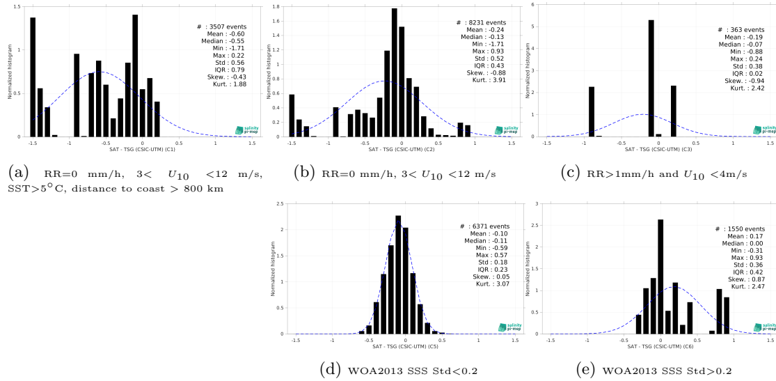
Figure 15: Normalized histogram of \Delta\text{SSS} (Aquarius SSS L2 OR v5 (NASA-GSFC) - TSG (CSIC-UTM)) for 5 different subdatasets corresponding to: RR=0 mm/h, 3 < U_{10} < 12 m/s, SST > 5^\circ\text{C} , distance to coast > 800 km (a), RR=0 mm/h, 3 < U_{10} < 12 m/s (b), RR > 1 mm/h and U_{10} < 4 m/s (c), WOA2013 SSS Std < 0.2 (d), WOA2013 SSS Std > 0.2 (e).
