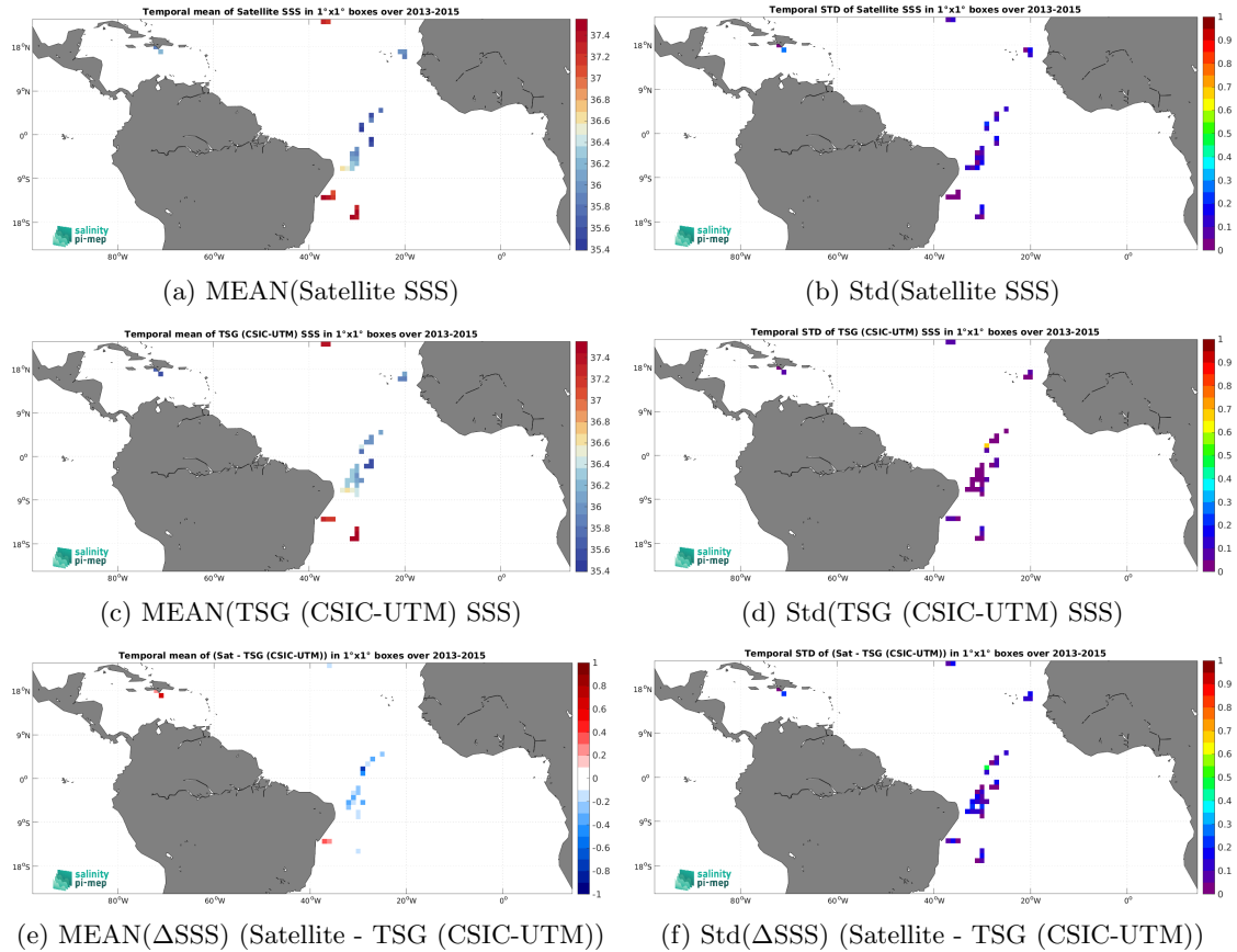
Figure 7: Temporal mean (left) and Std (right) of SSS from Aquarius SSS L2 OR v5 (NASA-GSFC) (top), TSG (CSIC-UTM) (middle), and of \Delta SSS (Satellite - TSG (CSIC-UTM)). Only match-up pairs are used to generate these maps.
