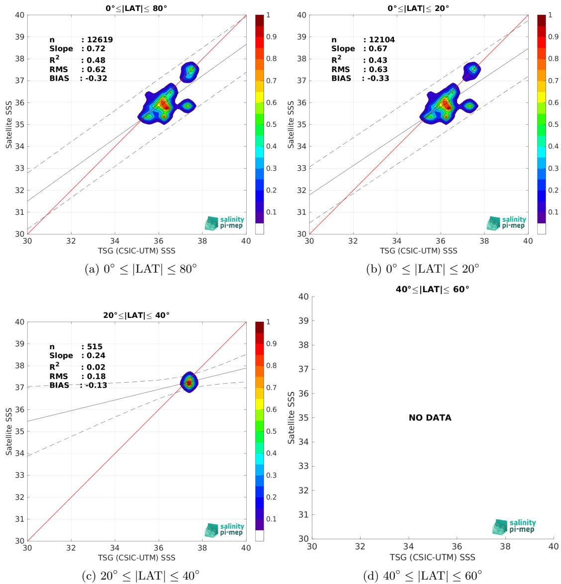
Figure 10: Contour maps of the concentration of Aquarius SSS L2 OR v5 (NASA-GSFC) SSS (y-axis) versus TSG (CSIC-UTM) SSS (x-axis) at match-up pairs for different latitude bands. For each plot, the red line shows x=y . The black thin and dashed lines indicate a linear fit through the data cloud and the \pm 95\% confidence levels, respectively. The number match-up pairs n , the slope and R^2 coefficient of the linear fit, the root mean square (RMS) and the mean bias between satellite and in situ data are indicated for each latitude band in each plots.
