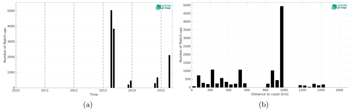
Figure 2: Number of match-ups between TSG (CSIC-UTM) and Aquarius SSS L2 OR v5 (NASA-GSFC) SSS as a function of time (a) and as function of the distance to coast (b) over the Tropical Atlantic Ocean Pi-MEP region and for the full satellite product period.
