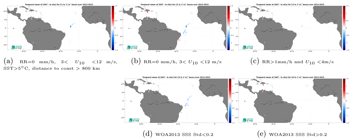
Figure 14: Temporal mean gridded over spatial boxes of size 1^\circ \times 1^\circ of \Delta SSS (Aquarius SSS L2 OR v5 (NASA-GSFC) - TSG (CSIC-UTM)) for 5 different subdatasets corresponding to:RR=0 mm/h, 3 < U_{10} < 12 m/s, SST >5^\circ\text{C} , distance to coast > 800 km (a), RR=0 mm/h, 3 < U_{10} < 12 m/s (b), RR >1 mm/h and U_{10} < 4 m/s (c), WOA2013 SSS Std <0.2 (d), WOA2013 SSS Std >0.2 (e).
