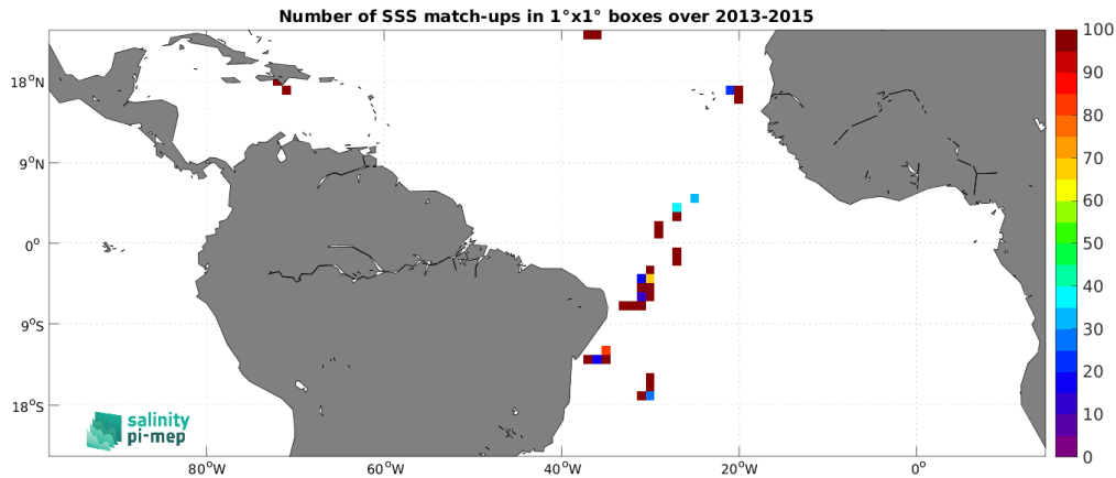
Figure 5: Number of SSS match-ups between TSG (CSIC-UTM) SSS and the Aquarius SSS L2 OR v5 (NASA-GSFC) SSS product for the Tropical Atlantic Ocean Pi-MEP region over 1^\circ \times 1^\circ boxes and for the full satellite product period.
