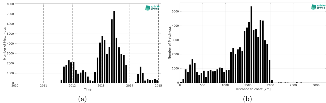
Figure 2: Number of match-ups between Surface drifters and Aquarius SSS L2 OR v5 (NASA-GSFC) SSS as a function of time (a) and as function of the distance to coast (b) over the Tropical Atlantic Ocean Pi-MEP region and for the full satellite product period.
