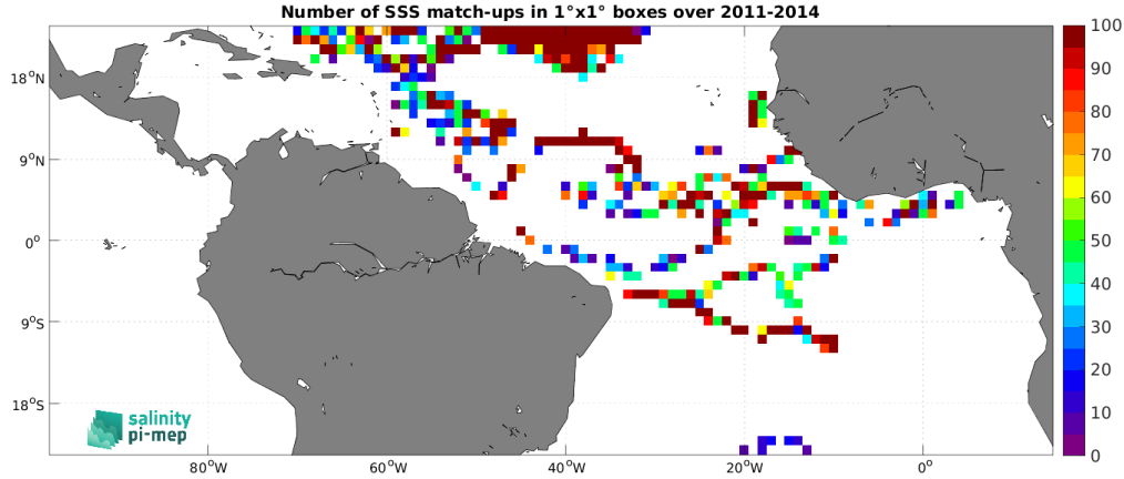
Figure 4: Number of SSS match-ups between Surface drifters SSS and the Aquarius SSS L2 OR v5 (NASA-GSFC) SSS product for the Tropical Atlantic Ocean Pi-MEP region over 1^\circ \times 1^\circ boxes and for the full satellite product period.
