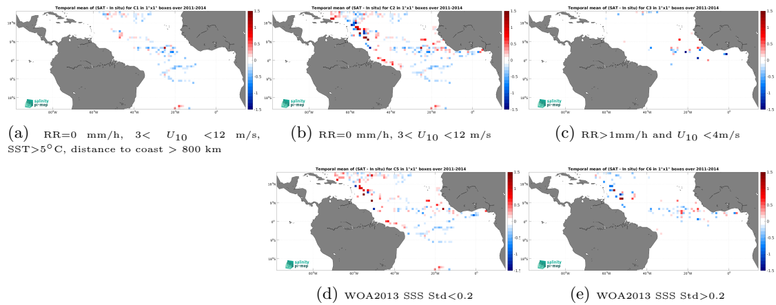
Figure 13: Temporal mean gridded over spatial boxes of size 1^\circ \times 1^\circ of \Delta\text{SSS} (Aquarius SSS L2 OR v5 (NASA-GSFC) - Surface drifters) for 5 different subdatasets corresponding to:RR=0 mm/h, 3 < U_{10} < 12 m/s, SST >5^\circ\text{C} , distance to coast > 800 km (a), RR=0 mm/h, 3 < U_{10} < 12 m/s (b), RR >1 mm/h and U_{10} < 4 m/s (c), WOA2013 SSS Std <0.2 (d), WOA2013 SSS Std >0.2 (e).
