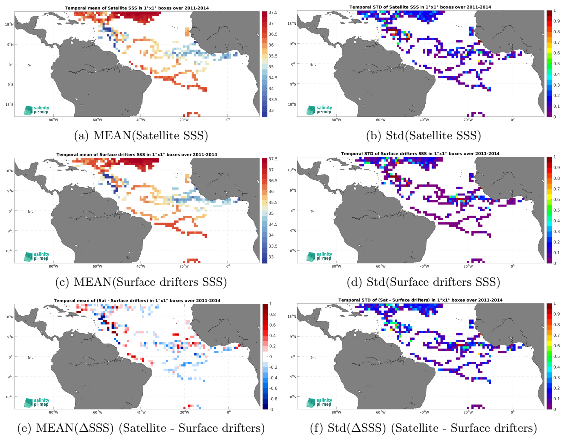
Figure 6: Temporal mean (left) and Std (right) of SSS from Aquarius SSS L2 OR v5 (NASA-GSFC) (top), Surface drifters (middle), and of \Delta SSS (Satellite - Surface drifters). Only match-up pairs are used to generate these maps.
