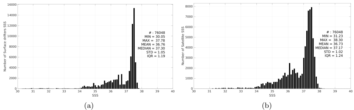
Figure 3: Histograms of SSS from Surface drifters (a) and Aquarius SSS L2 OR v5 (NASA-GSFC) (b) considering all match-up pairs per bins of 0.1 over the Tropical Atlantic Ocean Pi-MEP region and for the full satellite product period.
