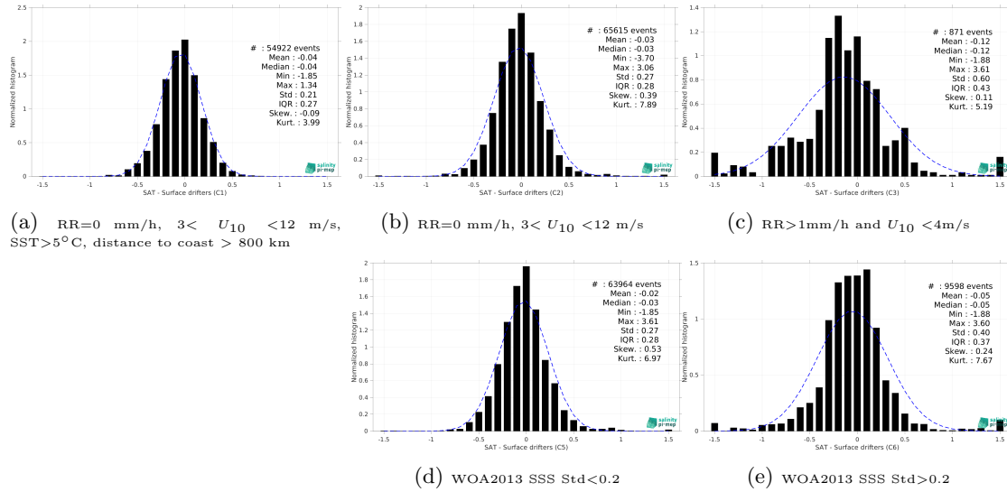
Figure 12: Normalized histogram of \Delta\text{SSS} (Aquarius SSS L2 OR v5 (NASA-GSFC) - Surface drifters) for 5 different subdatasets corresponding to: RR=0 mm/h, 3 < U_{10} < 12 m/s, SST>5°C, distance to coast > 800 km (a), RR=0 mm/h, 3 < U_{10} < 12 m/s (b), RR>1mm/h and U_{10} < 4 m/s (c), WOA2013 SSS Std<0.2 (d), WOA2013 SSS Std>0.2 (e).
