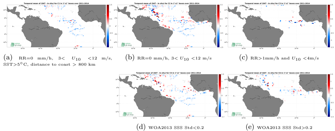
Figure 11: Temporal mean gridded over spatial boxes of size 1^\circ \times 1^\circ of \Delta SSS (Aquarius SSS L2 OR v5 (NASA-GSFC) - Surface drifters) for 5 different subdatasets corresponding to:RR=0 mm/h, 3 < U_{10} < 12 m/s, SST >5^\circ\text{C} , distance to coast > 800 km (a), RR=0 mm/h, 3 < U_{10} < 12 m/s (b), RR >1 mm/h and U_{10} < 4 m/s (c), WOA2013 SSS Std <0.2 (d), WOA2013 SSS Std >0.2 (e).
