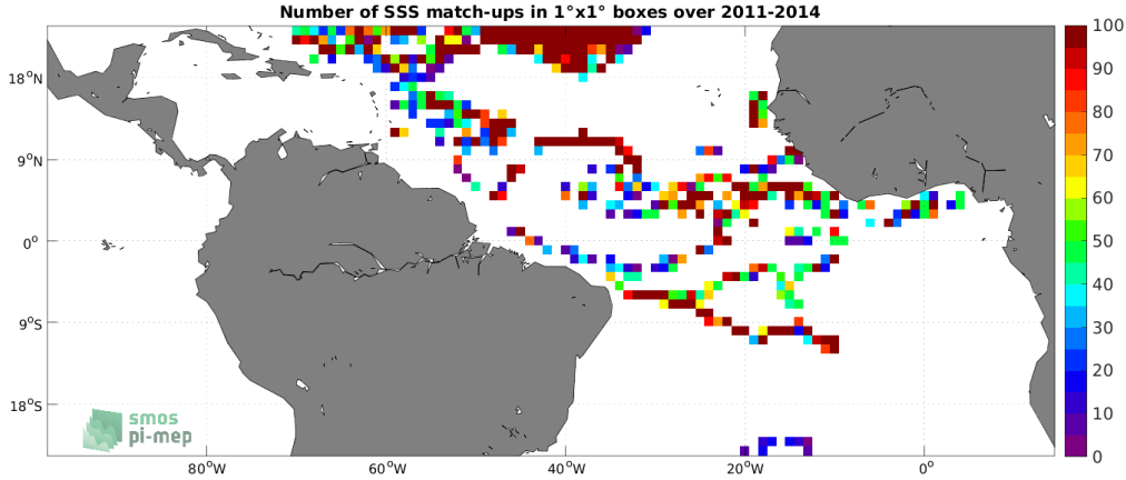
Figure 3: Number of SSS match-ups between Surface drifters SSS and the Aquarius SSS L2 OR v5 (NASA-GSFC) SSS product for the Tropical Atlantic Ocean Pi-MEP region over 1^\circ \times 1^\circ boxes and for the full satellite product period.
