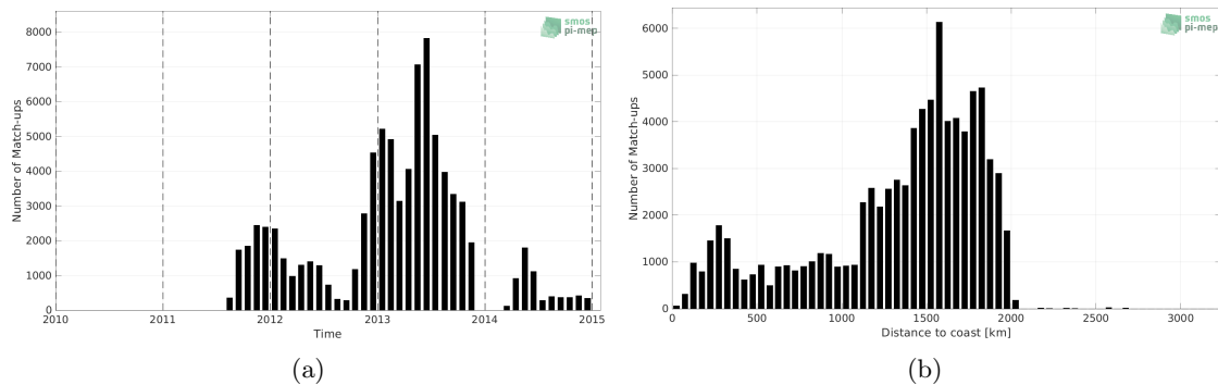
Figure 1: Number of match-ups between Surface drifters and Aquarius SSS L2 OR v5 (NASA-GSFC) SSS as a function of time (a) and as function of the distance to coast (b) over the Tropical Atlantic Ocean Pi-MEP region and for the full satellite product period.
