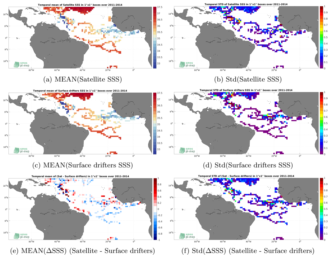
Figure 5: Temporal mean (left) and Std (right) of SSS from Aquarius SSS L2 OR v5 (NASA-GSFC) (top), Surface drifters (middle), and of \Delta SSS (Satellite - Surface drifters). Only match-up pairs are used to generate these maps.
