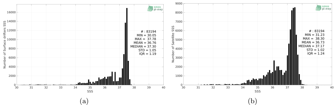
Figure 2: Histograms of SSS from Surface drifters (a) and Aquarius SSS L2 OR v5 (NASA-GSFC) (b) considering all match-up pairs per bins of 0.1 over the Tropical Atlantic Ocean Pi-MEP region and for the full satellite product period.
