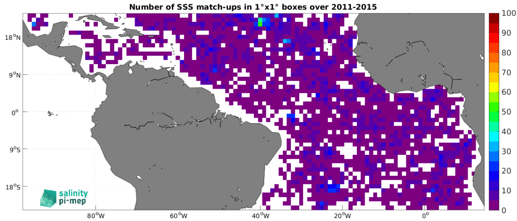
Figure 4: Number of SSS match-ups between Argo SSS and the Aquarius SSS L2 OR v5 (NASA-GSFC) SSS product for the Tropical Atlantic Ocean Pi-MEP region over 1^\circ \times 1^\circ boxes and for the full satellite product period.
