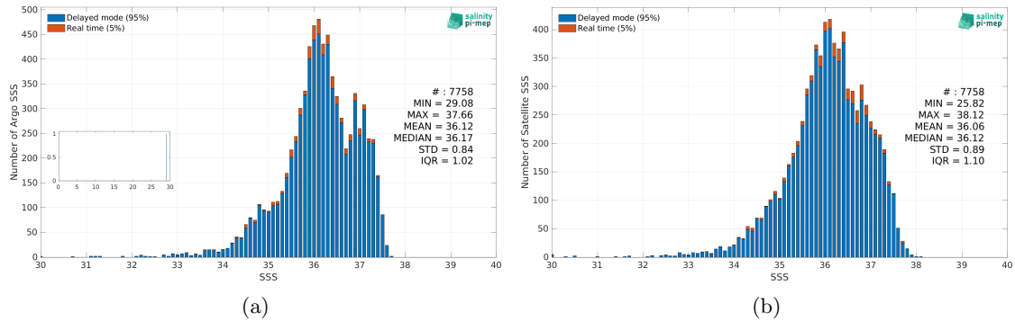
Figure 2: Histograms of SSS from Argo (a) and Aquarius SSS L2 OR v5 (NASA-GSFC) (b) considering all match-up pairs per bins of 0.1 over the Tropical Atlantic Ocean Pi-MEP region and for the full satellite product period.
