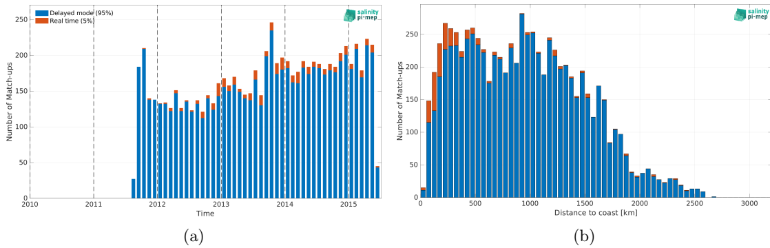
Figure 1: Number of match-ups between Argo and Aquarius SSS L2 OR v5 (NASA-GSFC) SSS as a function of time (a) and as function of the distance to coast (b) over the Tropical Atlantic Ocean Pi-MEP region and for the full satellite product period.
