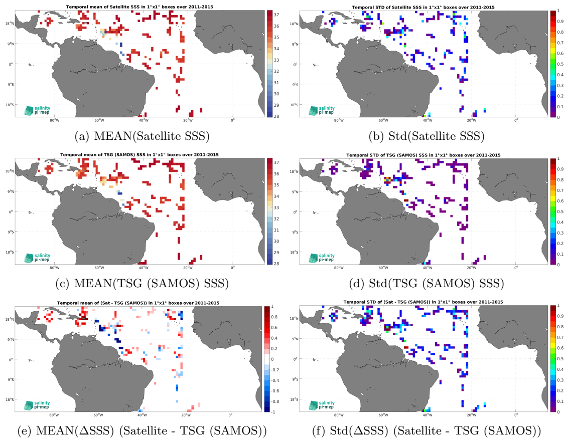
Figure 7: Temporal mean (left) and Std (right) of SSS from Aquarius SSS L2 CAP v5 (JPL) (top), TSG (SAMOS) (middle), and of \Delta SSS (Satellite - TSG (SAMOS)). Only match-up pairs are used to generate these maps.
