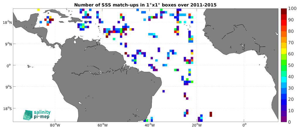
Figure 5: Number of SSS match-ups between TSG (SAMOS) SSS and the Aquarius SSS L2 CAP v5 (JPL) SSS product for the Tropical Atlantic Ocean Pi-MEP region over 1^\circ \times 1^\circ boxes and for the full satellite product period.
