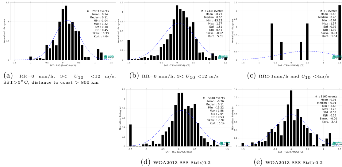
Figure 15: Normalized histogram of \Delta\text{SSS} (Aquarius SSS L2 CAP v5 (JPL) - TSG (SAMOS)) for 5 different subdatasets corresponding to: RR=0 mm/h, 3 < U_{10} < 12 m/s, SST>5°C, distance to coast > 800 km (a), RR=0 mm/h, 3 < U_{10} < 12 m/s (b), RR>1mm/h and U_{10} < 4 m/s (c), WOA2013 SSS Std<0.2 (d), WOA2013 SSS Std>0.2 (e).
