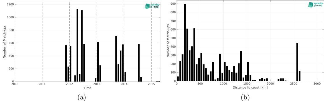
Figure 2: Number of match-ups between TSG (SAMOS) and Aquarius SSS L2 CAP v5 (JPL) SSS as a function of time (a) and as function of the distance to coast (b) over the Tropical Atlantic Ocean Pi-MEP region and for the full satellite product period.
