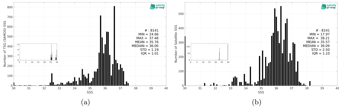
Figure 3: Histograms of SSS from TSG (SAMOS) (a) and Aquarius SSS L2 CAP v5 (JPL) (b) considering all match-up pairs per bins of 0.1 over the Tropical Atlantic Ocean Pi-MEP region and for the full satellite product period.
