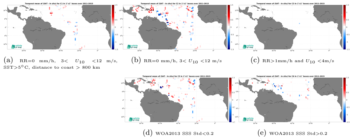
Figure 12: Temporal mean gridded over spatial boxes of size 1^\circ \times 1^\circ of \Delta\text{SSS} (Aquarius SSS L2 CAP v5 (JPL) - TSG (SAMOS)) for 5 different subdatasets corresponding to:RR=0 mm/h, 3 < U_{10} < 12 m/s, SST >5^\circ\text{C} , distance to coast > 800 km (a), RR=0 mm/h, 3 < U_{10} < 12 m/s (b), RR >1 mm/h and U_{10} < 4 m/s (c), WOA2013 SSS Std <0.2 (d), WOA2013 SSS Std >0.2 (e).
