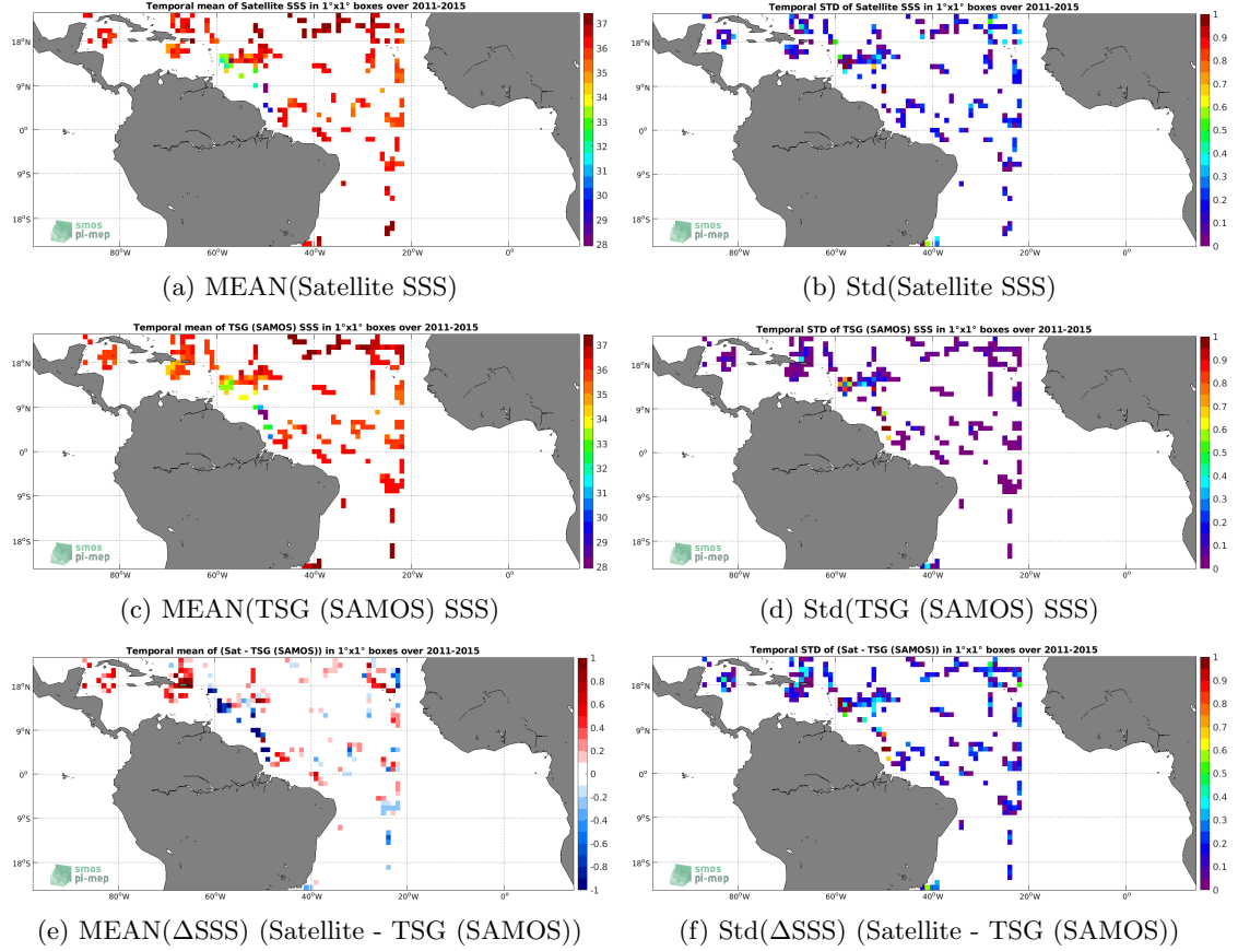
Figure 6: Temporal mean (left) and Std (right) of SSS from Aquarius SSS L2 CAP v5 (JPL) (top), TSG (SAMOS) (middle), and of \Delta\text{SSS} (Satellite - TSG (SAMOS)). Only match-up pairs are used to generate these maps.
