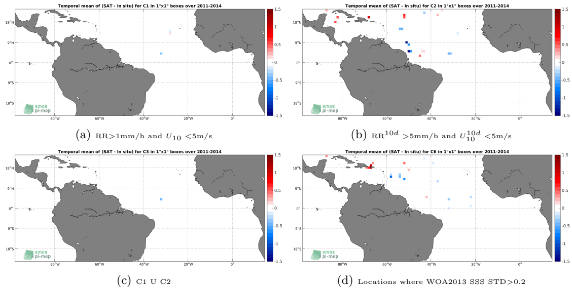
Figure 12: Temporal mean gridded over spatial boxes of size 1^\circ \times 1^\circ of \Delta\text{SSS} (Aquarius-L2-JPL-V5 - TSG-SAMOS) for 4 different subdatasets corresponding to: RR > 1\text{mm/h} and U_{10} < 5\text{m/s} (a), RR^{10d} > 5\text{mm/h} and U_{10}^{10d} < 5\text{m/s} (b), C1 U C2 (c), Locations where WOA2013 SSS STD > 0.2 (d).
