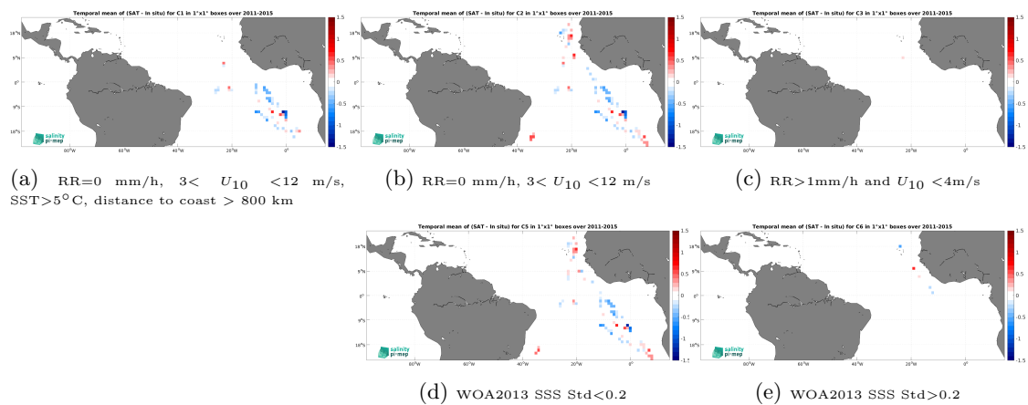
Figure 14: Temporal mean gridded over spatial boxes of size 1^\circ \times 1^\circ of \Delta\text{SSS} (Aquarius SSS L2 CAP v5 (JPL) - TSG (Polarstern)) for 5 different subdatasets corresponding to:RR=0 mm/h, 3 < U_{10} < 12 m/s, SST >5^\circ\text{C} , distance to coast > 800 km (a), RR=0 mm/h, 3 < U_{10} < 12 m/s (b), RR >1 mm/h and U_{10} < 4 m/s (c), WOA2013 SSS Std <0.2 (d), WOA2013 SSS Std >0.2 (e).
