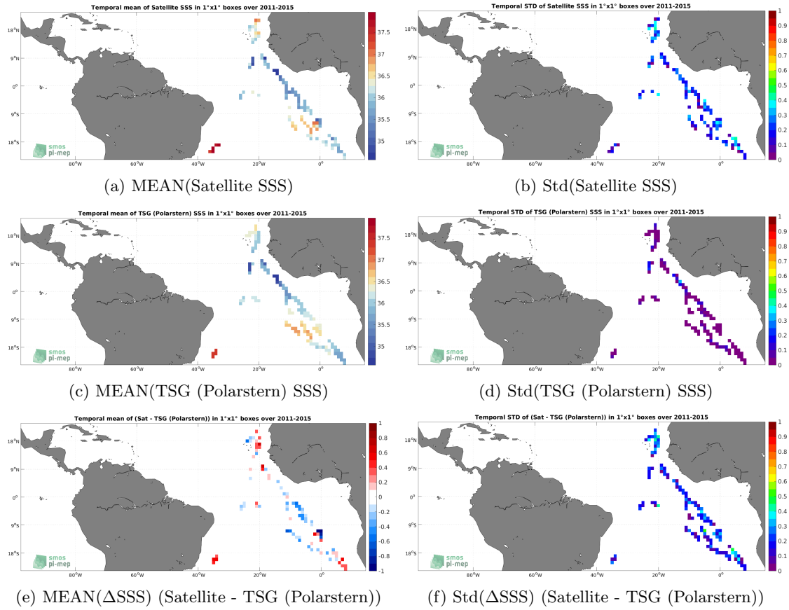
Figure 6: Temporal mean (left) and Std (right) of SSS from Aquarius SSS L2 CAP v5 (JPL) (top), TSG (Polarstern) (middle), and of \Delta SSS (Satellite - TSG (Polarstern)). Only match-up pairs are used to generate these maps.
