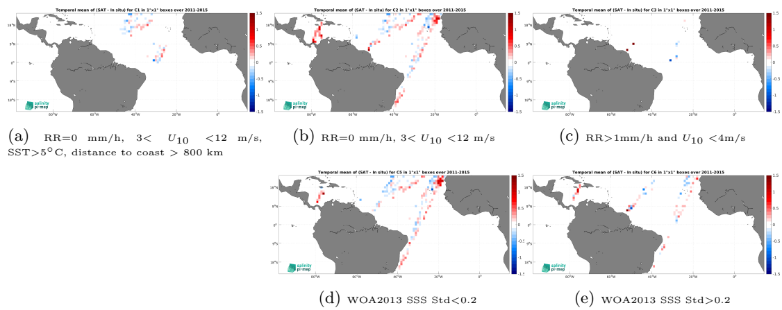
Figure 14: Temporal mean gridded over spatial boxes of size 1^\circ \times 1^\circ of \Delta\text{SSS} (Aquarius SSS L2 CAP v5 (JPL) - TSG (LEGOS-DM)) for 5 different subdatasets corresponding to:RR=0 mm/h, 3 < U_{10} < 12 m/s, SST>5°C, distance to coast > 800 km (a), RR=0 mm/h, 3 < U_{10} < 12 m/s (b), RR>1mm/h and U_{10} < 4 m/s (c), WOA2013 SSS Std<0.2 (d), WOA2013 SSS Std>0.2 (e).
