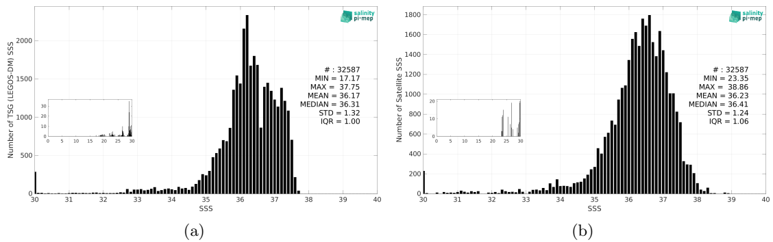
Figure 3: Histograms of SSS from TSG (LEGOS-DM) (a) and Aquarius SSS L2 CAP v5 (JPL) (b) considering all match-up pairs per bins of 0.1 over the Tropical Atlantic Ocean Pi-MEP region and for the full satellite product period.
