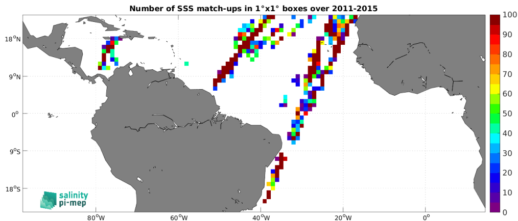
Figure 5: Number of SSS match-ups between TSG (LEGOS-DM) SSS and the Aquarius SSS L2 CAP v5 (JPL) SSS product for the Tropical Atlantic Ocean Pi-MEP region over 1^\circ \times 1^\circ boxes and for the full satellite product period.
