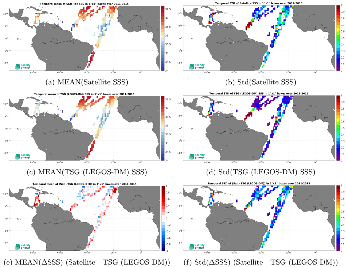
Figure 7: Temporal mean (left) and Std (right) of SSS from Aquarius SSS L2 CAP v5 (JPL) (top), TSG (LEGOS-DM) (middle), and of \Delta SSS (Satellite - TSG (LEGOS-DM)). Only match-up pairs are used to generate these maps.
