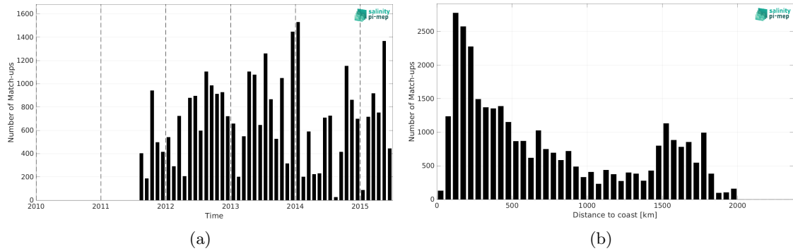
Figure 2: Number of match-ups between TSG (LEGOS-DM) and Aquarius SSS L2 CAP v5 (JPL) SSS as a function of time (a) and as function of the distance to coast (b) over the Tropical Atlantic Ocean Pi-MEP region and for the full satellite product period.
