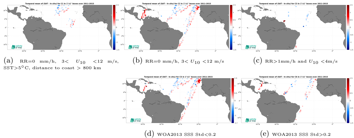
Figure 12: Temporal mean gridded over spatial boxes of size 1^\circ \times 1^\circ of \Delta\text{SSS} (Aquarius SSS L2 CAP v5 (JPL) - TSG (LEGOS-DM)) for 5 different subdatasets corresponding to:RR=0 mm/h, 3 < U_{10} < 12 m/s, SST >5^\circ\text{C} , distance to coast > 800 km (a), RR=0 mm/h, 3 < U_{10} < 12 m/s (b), RR >1 mm/h and U_{10} < 4 m/s (c), WOA2013 SSS Std <0.2 (d), WOA2013 SSS Std >0.2 (e).
