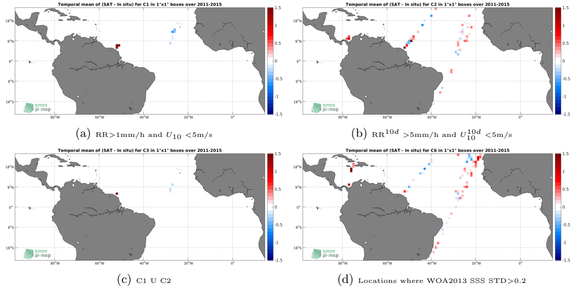
Figure 12: Temporal mean gridded over spatial boxes of size 1^\circ \times 1^\circ of \Delta SSS (Aquarius-L2-JPL-V5 - TSG-LEGOS-DM) for 4 different subdatasets corresponding to:RR>1mm/h and U_{10} < 5\text{m/s} (a), RR^{10d} > 5\text{mm/h} and U_{10}^{10d} < 5\text{m/s} (b), C1 U C2 (c),Locations where WOA2013 SSS STD>0.2 (d).
