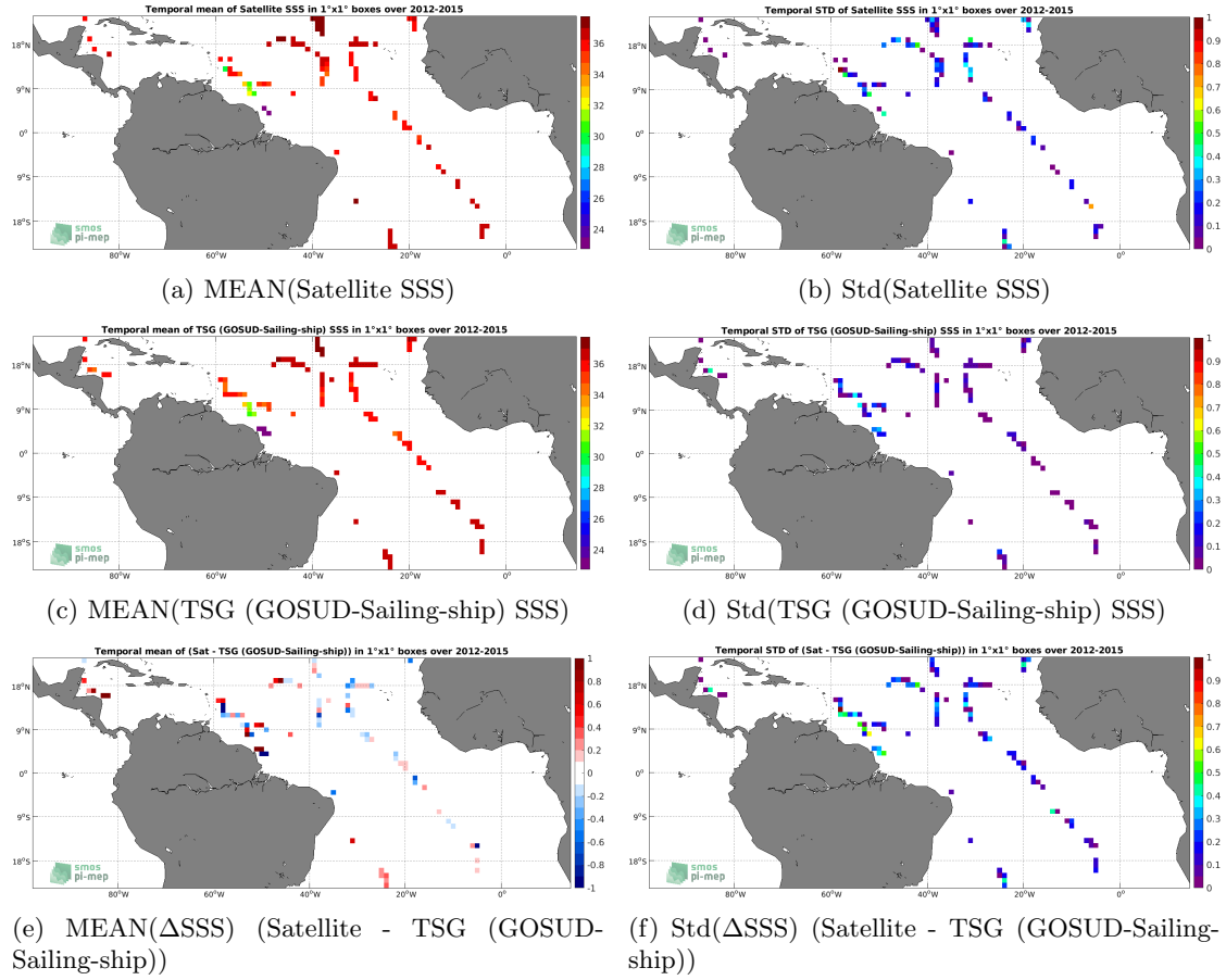
Figure 6: Temporal mean (left) and Std (right) of SSS from Aquarius SSS L2 CAP v5 (JPL) (top), TSG (GOSUD-Sailing-ship) (middle), and of \Delta SSS (Satellite - TSG (GOSUD-Sailing-ship)). Only match-up pairs are used to generate these maps.
