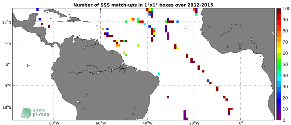
Figure 4: Number of SSS match-ups between TSG (GOSUD-Sailing-ship) SSS and the Aquarius SSS L2 CAP v5 (JPL) SSS product for the Tropical Atlantic Ocean Pi-MEP region over 1^\circ \times 1^\circ boxes and for the full satellite product period.
