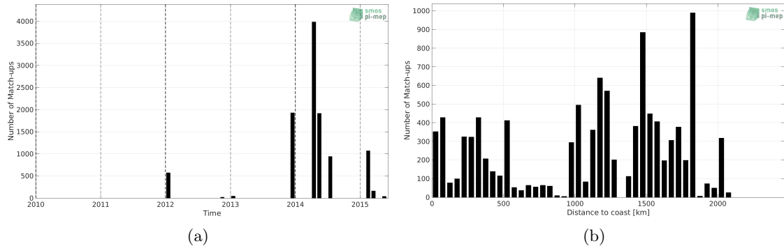
Figure 1: Number of match-ups between TSG (GOSUD-Sailing-ship) and Aquarius SSS L2 CAP v5 (JPL) SSS as a function of time (a) and as function of the distance to coast (b) over the Tropical Atlantic Ocean Pi-MEP region and for the full satellite product period.
