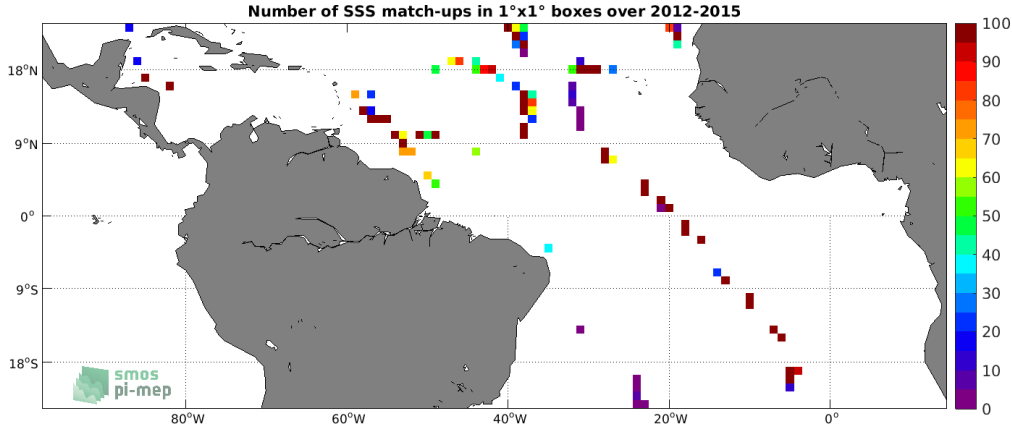
Figure 4: Number of SSS match-ups between TSG (GOSUD-Sailing-ship) SSS and the Aquarius SSS L2 CAP v5 (JPL) SSS product for the Tropical Atlantic Ocean Pi-MEP region over 1°x1° boxes and for the full satellite product period.
