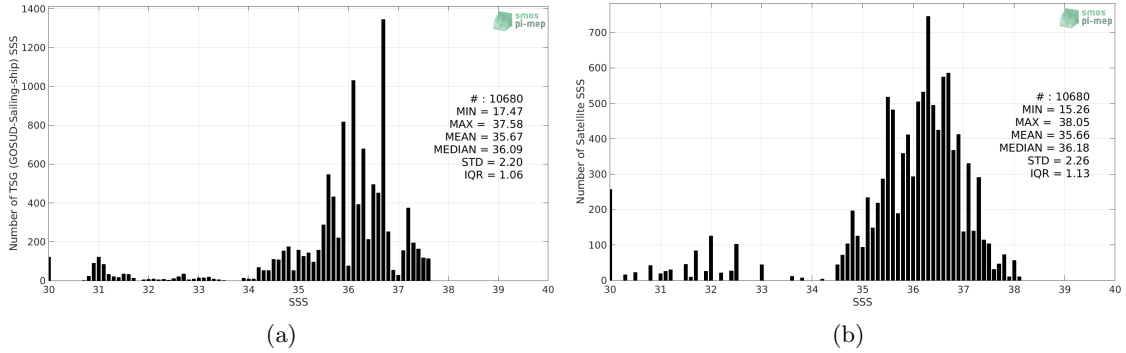
Figure 2: Histograms of SSS from TSG (GOSUD-Sailing-ship) (a) and Aquarius SSS L2 CAP v5 (JPL) (b) considering all match-up pairs per bins of 0.1 over the Tropical Atlantic Ocean Pi-MEP region and for the full satellite product period.
