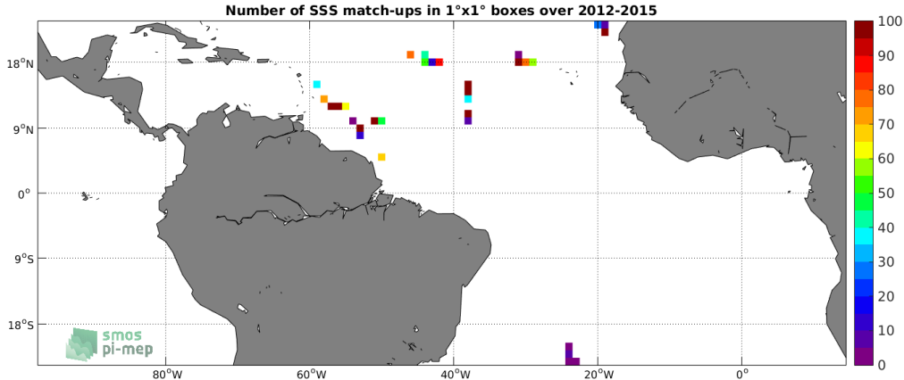
Figure 4: Number of SSS match-ups between TSG-GOSUD-Sailing-ship SSS and the Aquarius-L2-JPL-V5 SSS product for the Tropical Atlantic Ocean Pi-MEP region over 1^\circ \times 1^\circ boxes and for the full satellite product period.
