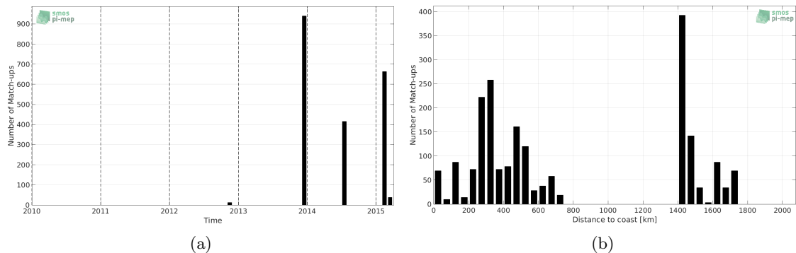
Figure 1: Number of match-ups between TSG-GOSUD-Sailing-ship and Aquarius-L2-JPL-V5 SSS as a function of time (a) and as function of the distance to coast (b) over the Tropical Atlantic Ocean Pi-MEP region and for the full satellite product period.
