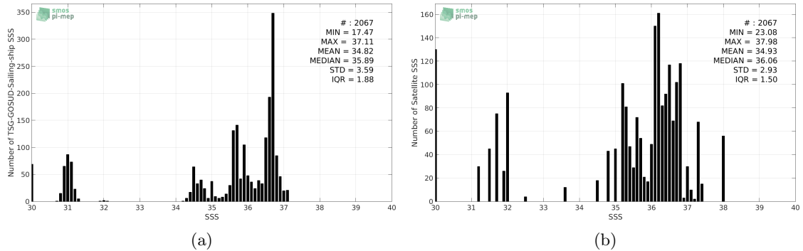
Figure 2: Histograms of SSS from TSG-GOSUD-Sailing-ship (a) and Aquarius-L2-JPL-V5 (b) considering all match-up pairs per bins of 0.1 over the Tropical Atlantic Ocean Pi-MEP region and for the full satellite product period.
