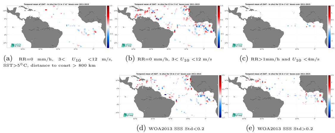
Figure 14: Temporal mean gridded over spatial boxes of size 1^\circ \times 1^\circ of \Delta SSS (Aquarius SSS L2 CAP v5 (JPL) - TSG (GOSUD-Research-vessel)) for 5 different subdatasets corresponding to:RR=0 mm/h, 3 < U_{10} < 12 m/s, SST >5^\circ\text{C} , distance to coast > 800 km (a), RR=0 mm/h, 3 < U_{10} < 12 m/s (b), RR >1 mm/h and U_{10} < 4 m/s (c), WOA2013 SSS Std <0.2 (d), WOA2013 SSS Std >0.2 (e).
