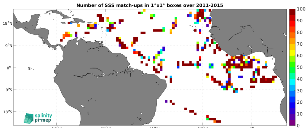
Figure 5: Number of SSS match-ups between TSG (GOSUD-Research-vessel) SSS and the Aquarius SSS L2 CAP v5 (JPL) SSS product for the Tropical Atlantic Ocean Pi-MEP region over 1^\circ \times 1^\circ boxes and for the full satellite product period.
