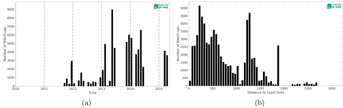
Figure 2: Number of match-ups between TSG (GOSUD-Research-vessel) and Aquarius SSS L2 CAP v5 (JPL) SSS as a function of time (a) and as function of the distance to coast (b) over the Tropical Atlantic Ocean Pi-MEP region and for the full satellite product period.
