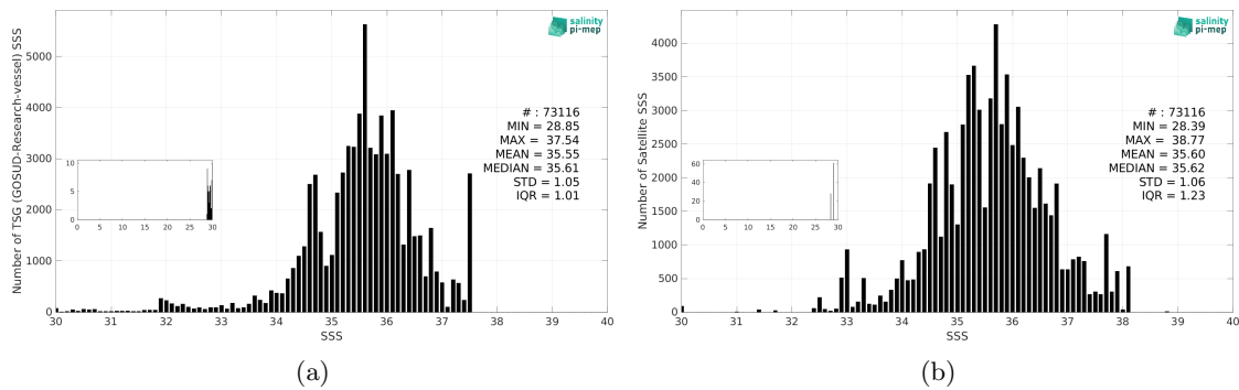
Figure 3: Histograms of SSS from TSG (GOSUD-Research-vessel) (a) and Aquarius SSS L2 CAP v5 (JPL) (b) considering all match-up pairs per bins of 0.1 over the Tropical Atlantic Ocean Pi-MEP region and for the full satellite product period.
