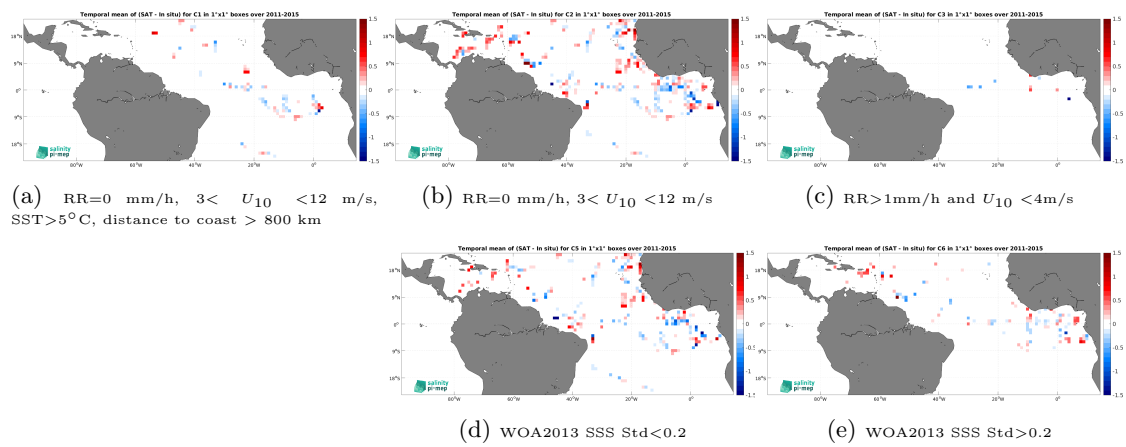
Figure 12: Temporal mean gridded over spatial boxes of size 1^\circ \times 1^\circ of \Delta SSS (Aquarius SSS L2 CAP v5 (JPL) - TSG (GOSUD-Research-vessel)) for 5 different subdatasets corresponding to:RR=0 mm/h, 3 < U_{10} < 12 m/s, SST >5^\circ\text{C} , distance to coast > 800 km (a), RR=0 mm/h, 3 < U_{10} < 12 m/s (b), RR >1 mm/h and U_{10} < 4 m/s (c), WOA2013 SSS Std <0.2 (d), WOA2013 SSS Std >0.2 (e).
