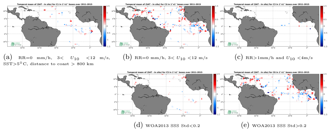
Figure 12: Temporal mean gridded over spatial boxes of size 1^\circ \times 1^\circ of \Delta\text{SSS} (Aquarius-L2-JPL-V5 - TSG-GOSUD-Research-vessel) for 5 different subdatasets corresponding to:RR=0 mm/h, 3 < U_{10} < 12 m/s, SST >5^\circ\text{C} , distance to coast > 800 km (a), RR=0 mm/h, 3 < U_{10} < 12 m/s (b), RR >1 mm/h and U_{10} < 4 m/s (c), WOA2013 SSS Std <0.2 (d), WOA2013 SSS Std >0.2 (e).
