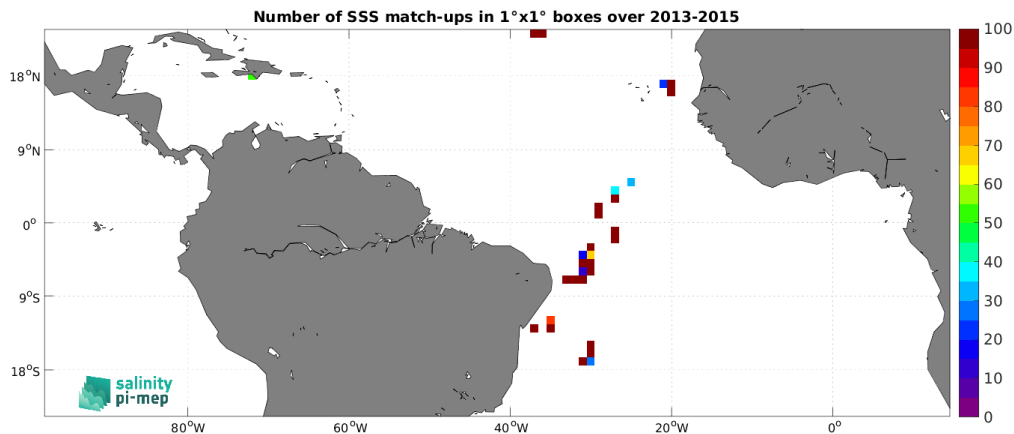
Figure 5: Number of SSS match-ups between TSG (CSIC-UTM) SSS and the Aquarius SSS L2 CAP v5 (JPL) SSS product for the Tropical Atlantic Ocean Pi-MEP region over 1^\circ \times 1^\circ boxes and for the full satellite product period.
