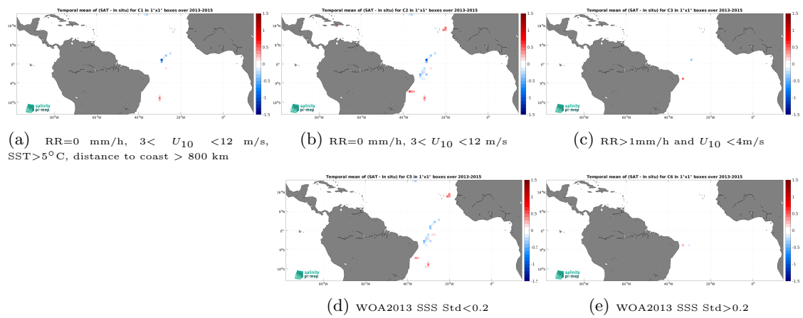
Figure 14: Temporal mean gridded over spatial boxes of size 1^\circ \times 1^\circ of \Delta SSS (Aquarius SSS L2 CAP v5 (JPL) - TSG (CSIC-UTM)) for 5 different subdatasets corresponding to:RR=0 mm/h, 3 < U_{10} < 12 m/s, SST >5^\circ\text{C} , distance to coast > 800 km (a), RR=0 mm/h, 3 < U_{10} < 12 m/s (b), RR >1 mm/h and U_{10} < 4 m/s (c), WOA2013 SSS Std <0.2 (d), WOA2013 SSS Std >0.2 (e).
