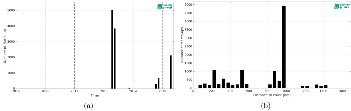
Figure 2: Number of match-ups between TSG (CSIC-UTM) and Aquarius SSS L2 CAP v5 (JPL) SSS as a function of time (a) and as function of the distance to coast (b) over the Tropical Atlantic Ocean Pi-MEP region and for the full satellite product period.
