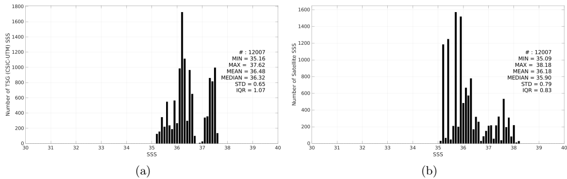
Figure 3: Histograms of SSS from TSG (CSIC-UTM) (a) and Aquarius SSS L2 CAP v5 (JPL) (b) considering all match-up pairs per bins of 0.1 over the Tropical Atlantic Ocean Pi-MEP region and for the full satellite product period.
