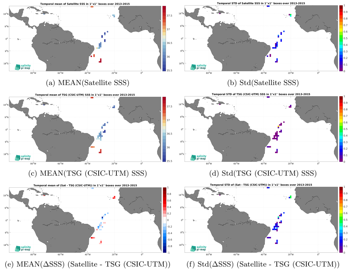
Figure 7: Temporal mean (left) and Std (right) of SSS from Aquarius SSS L2 CAP v5 (JPL) (top), TSG (CSIC-UTM) (middle), and of \Delta SSS (Satellite - TSG (CSIC-UTM)). Only match-up pairs are used to generate these maps.
