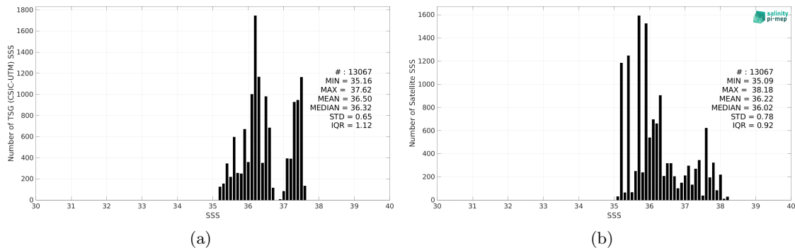
Figure 2: Histograms of SSS from TSG (CSIC-UTM) (a) and Aquarius SSS L2 CAP v5 (JPL) (b) considering all match-up pairs per bins of 0.1 over the Tropical Atlantic Ocean Pi-MEP region and for the full satellite product period.
