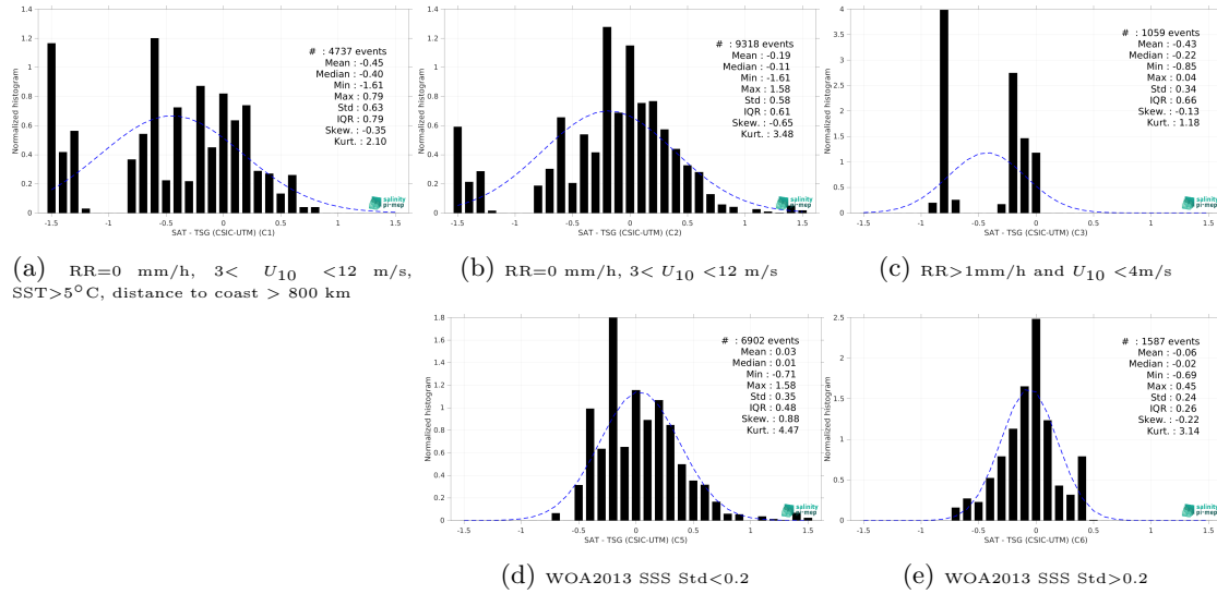
Figure 13: Normalized histogram of \Delta SSS (Aquarius SSS L2 CAP v5 (JPL) - TSG (CSIC-UTM)) for 5 different subdatasets corresponding to: RR=0 mm/h, 3 < U_{10} < 12 m/s, SST > 5°C, distance to coast > 800 km (a), RR=0 mm/h, 3 < U_{10} < 12 m/s (b), RR > 1mm/h and U_{10} < 4 m/s (c), WOA2013 SSS Std < 0.2 (d), WOA2013 SSS Std > 0.2 (e).
