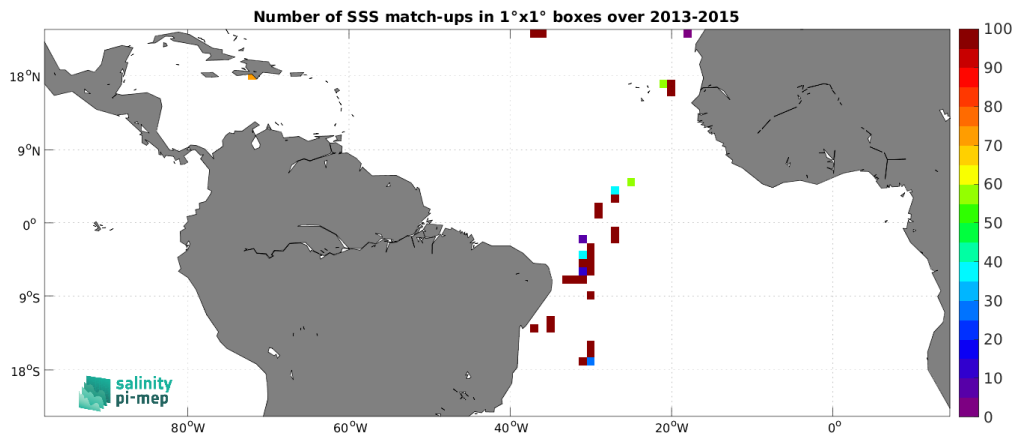
Figure 4: Number of SSS match-ups between TSG (CSIC-UTM) SSS and the Aquarius SSS L2 CAP v5 (JPL) SSS product for the Tropical Atlantic Ocean Pi-MEP region over 1^\circ \times 1^\circ boxes and for the full satellite product period.
