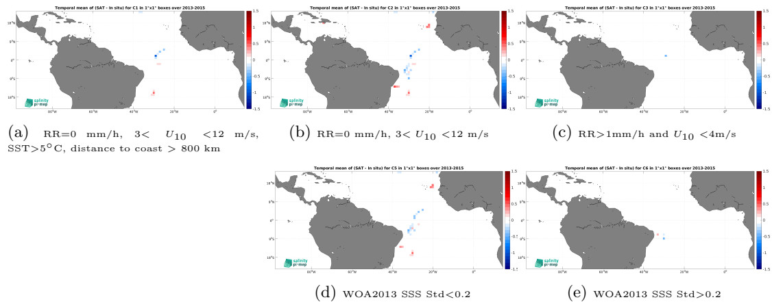
Figure 12: Temporal mean gridded over spatial boxes of size 1^\circ \times 1^\circ of \Delta SSS (Aquarius SSS L2 CAP v5 (JPL) - TSG (CSIC-UTM)) for 5 different subdatasets corresponding to:RR=0 mm/h, 3 < U_{10} < 12 m/s, SST >5^\circ\text{C} , distance to coast > 800 km (a), RR=0 mm/h, 3 < U_{10} < 12 m/s (b), RR >1 mm/h and U_{10} < 4 m/s (c), WOA2013 SSS Std <0.2 (d), WOA2013 SSS Std >0.2 (e).
