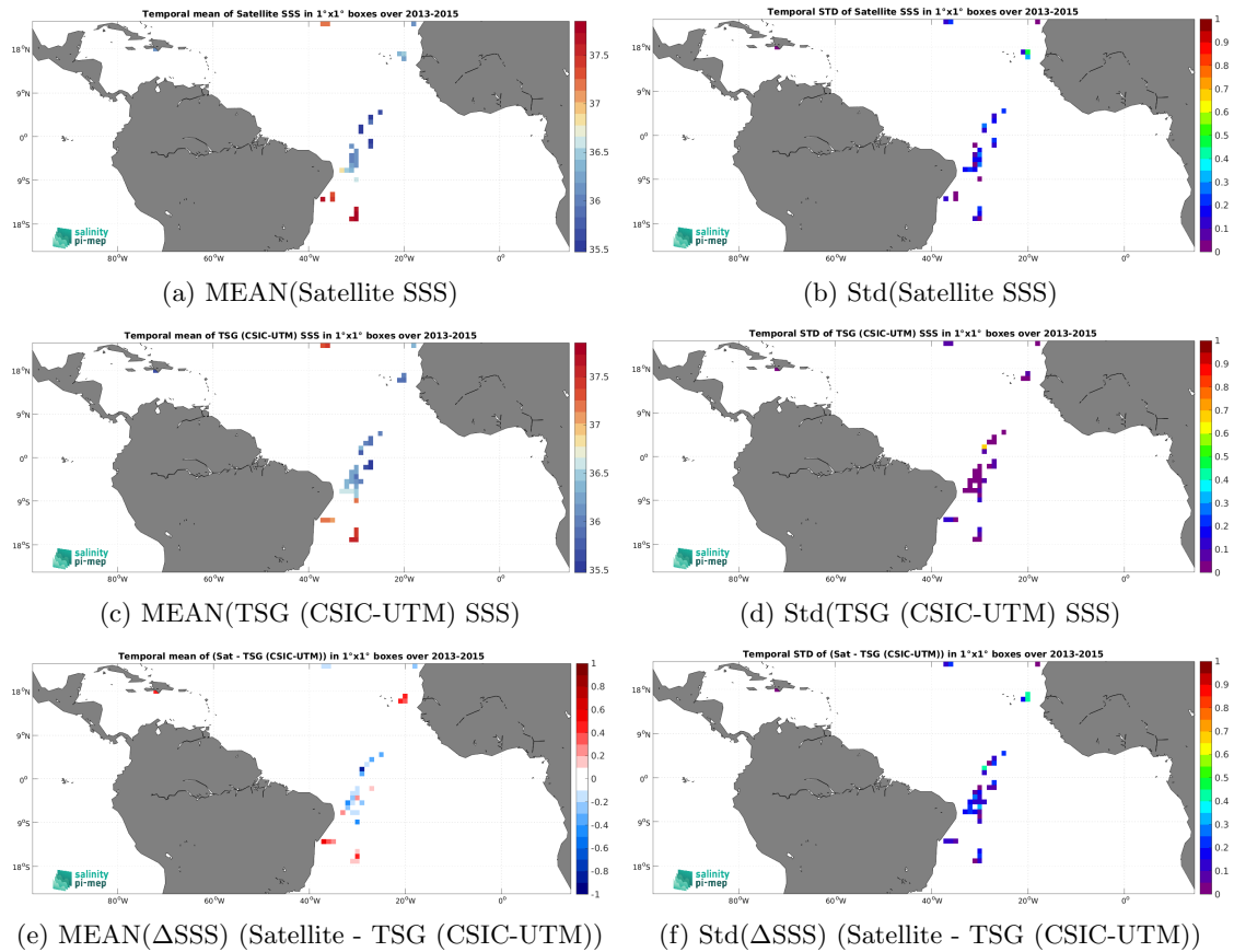
Figure 6: Temporal mean (left) and Std (right) of SSS from Aquarius SSS L2 CAP v5 (JPL) (top), TSG (CSIC-UTM) (middle), and of \Delta SSS (Satellite - TSG (CSIC-UTM)). Only match-up pairs are used to generate these maps.
