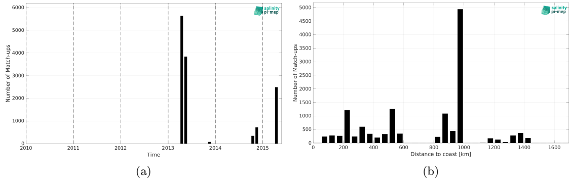
Figure 1: Number of match-ups between TSG (CSIC-UTM) and Aquarius SSS L2 CAP v5 (JPL) SSS as a function of time (a) and as function of the distance to coast (b) over the Tropical Atlantic Ocean Pi-MEP region and for the full satellite product period.
