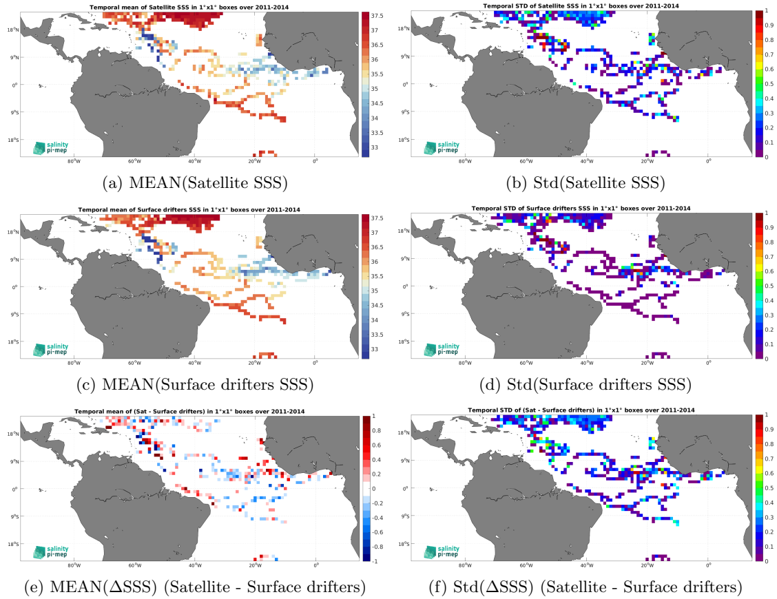
Figure 6: Temporal mean (left) and Std (right) of SSS from Aquarius SSS L2 CAP v5 (JPL) (top), Surface drifters (middle), and of \Delta SSS (Satellite - Surface drifters). Only match-up pairs are used to generate these maps.
