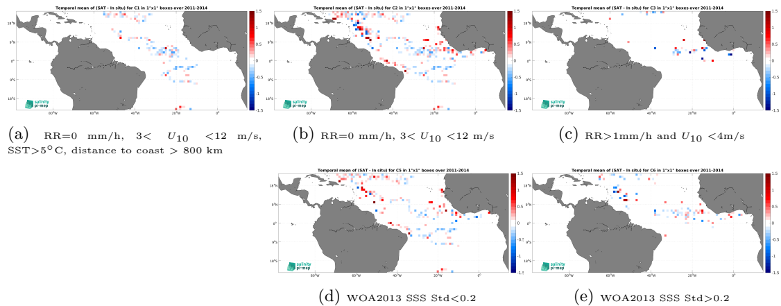
Figure 13: Temporal mean gridded over spatial boxes of size 1^\circ \times 1^\circ of \Delta SSS (Aquarius SSS L2 CAP v5 (JPL) - Surface drifters) for 5 different subdatasets corresponding to:RR=0 mm/h, 3 < U_{10} < 12 m/s, SST >5^\circ\text{C} , distance to coast > 800 km (a), RR=0 mm/h, 3 < U_{10} < 12 m/s (b), RR >1 mm/h and U_{10} < 4 m/s (c), WOA2013 SSS Std <0.2 (d), WOA2013 SSS Std >0.2 (e).
