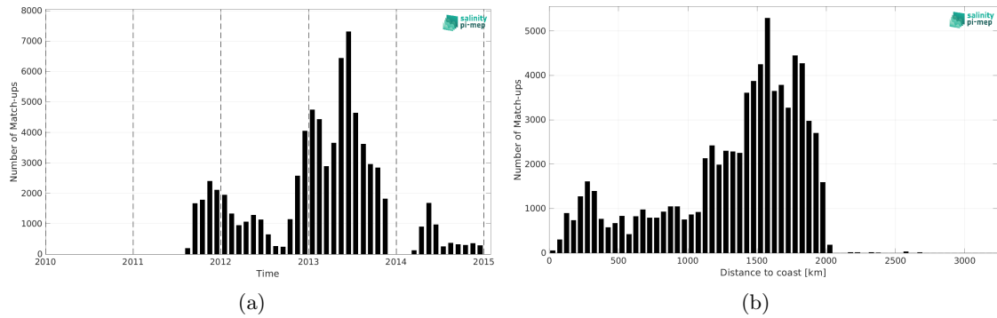
Figure 2: Number of match-ups between Surface drifters and Aquarius SSS L2 CAP v5 (JPL) SSS as a function of time (a) and as function of the distance to coast (b) over the Tropical Atlantic Ocean Pi-MEP region and for the full satellite product period.
