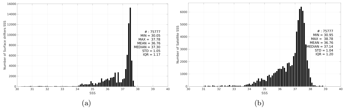
Figure 3: Histograms of SSS from Surface drifters (a) and Aquarius SSS L2 CAP v5 (JPL) (b) considering all match-up pairs per bins of 0.1 over the Tropical Atlantic Ocean Pi-MEP region and for the full satellite product period.
