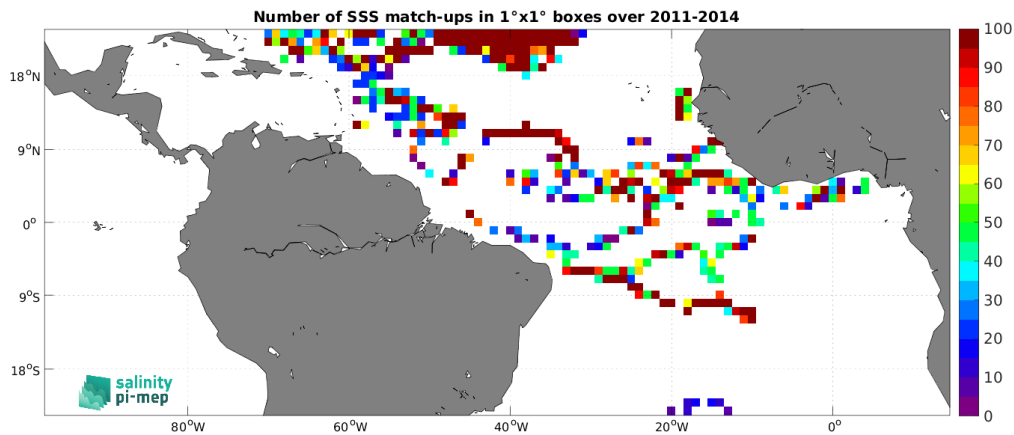
Figure 4: Number of SSS match-ups between Surface drifters SSS and the Aquarius SSS L2 CAP v5 (JPL) SSS product for the Tropical Atlantic Ocean Pi-MEP region over 1^\circ \times 1^\circ boxes and for the full satellite product period.
