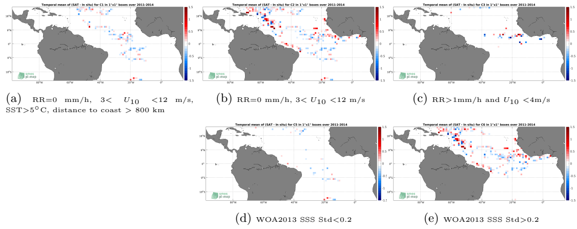
Figure 11: Temporal mean gridded over spatial boxes of size 1^\circ \times 1^\circ of \Delta\text{SSS} (Aquarius SSS L2 CAP v5 (JPL) - Surface drifters) for 5 different subdatasets corresponding to: \text{RR}=0 mm/h, 3 < U_{10} < 12 m/s, \text{SST} > 5^\circ\text{C} , distance to coast > 800 km (a), \text{RR}=0 mm/h, 3 < U_{10} < 12 m/s (b), \text{RR} > 1\text{mm/h} and U_{10} < 4\text{m/s} (c), WOA2013 SSS Std < 0.2 (d), WOA2013 SSS Std > 0.2 (e).
