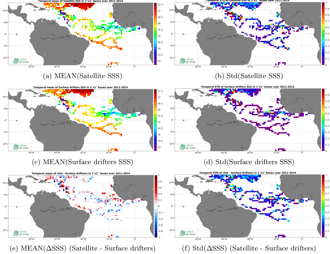
Figure 5: Temporal mean (left) and Std (right) of SSS from Aquarius SSS L2 CAP v5 (JPL) (top), Surface drifters (middle), and of \Delta\text{SSS} (Satellite - Surface drifters). Only match-up pairs are used to generate these maps.
