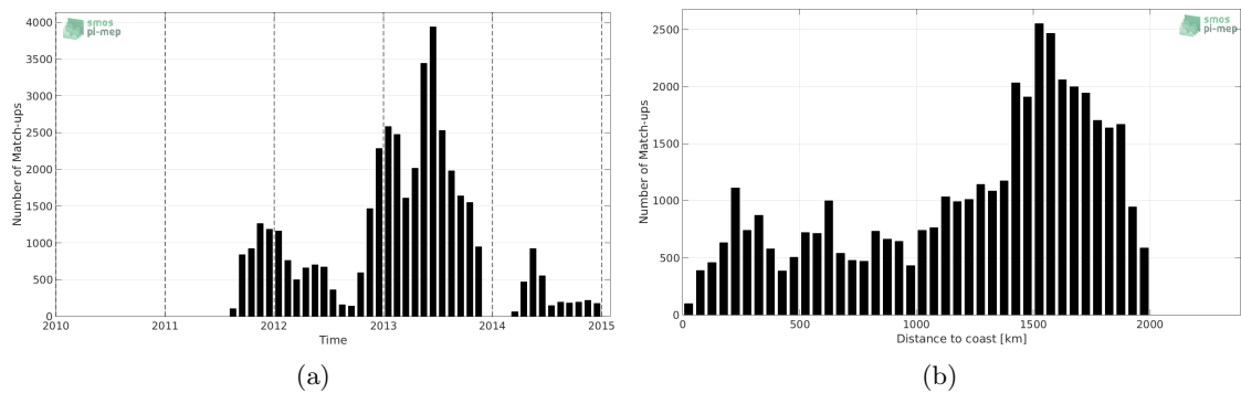
Figure 1: Number of match-ups between Surface drifters and Aquarius-L2-JPL-V5 SSS as a function of time (a) and as function of the distance to coast (b) over the Tropical Atlantic Ocean Pi-MEP region and for the full satellite product period.
