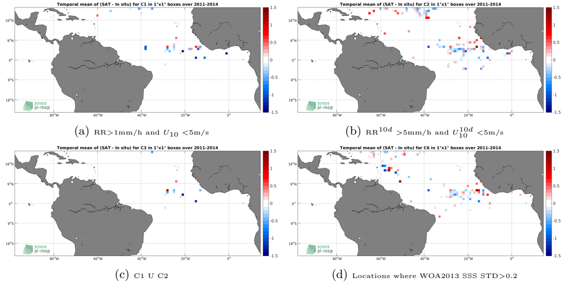
Figure 11: Temporal mean gridded over spatial boxes of size 1^\circ \times 1^\circ of \Delta SSS (Aquarius-L2-JPL-V5 - Surface drifters) for 4 different subdatasets corresponding to: RR > 1\text{mm/h} and U_{10} < 5\text{m/s} (a), RR^{10d} > 5\text{mm/h} and U_{10}^{10d} < 5\text{m/s} (b), C1 U C2 (c), Locations where WOA2013 SSS STD > 0.2 (d).
