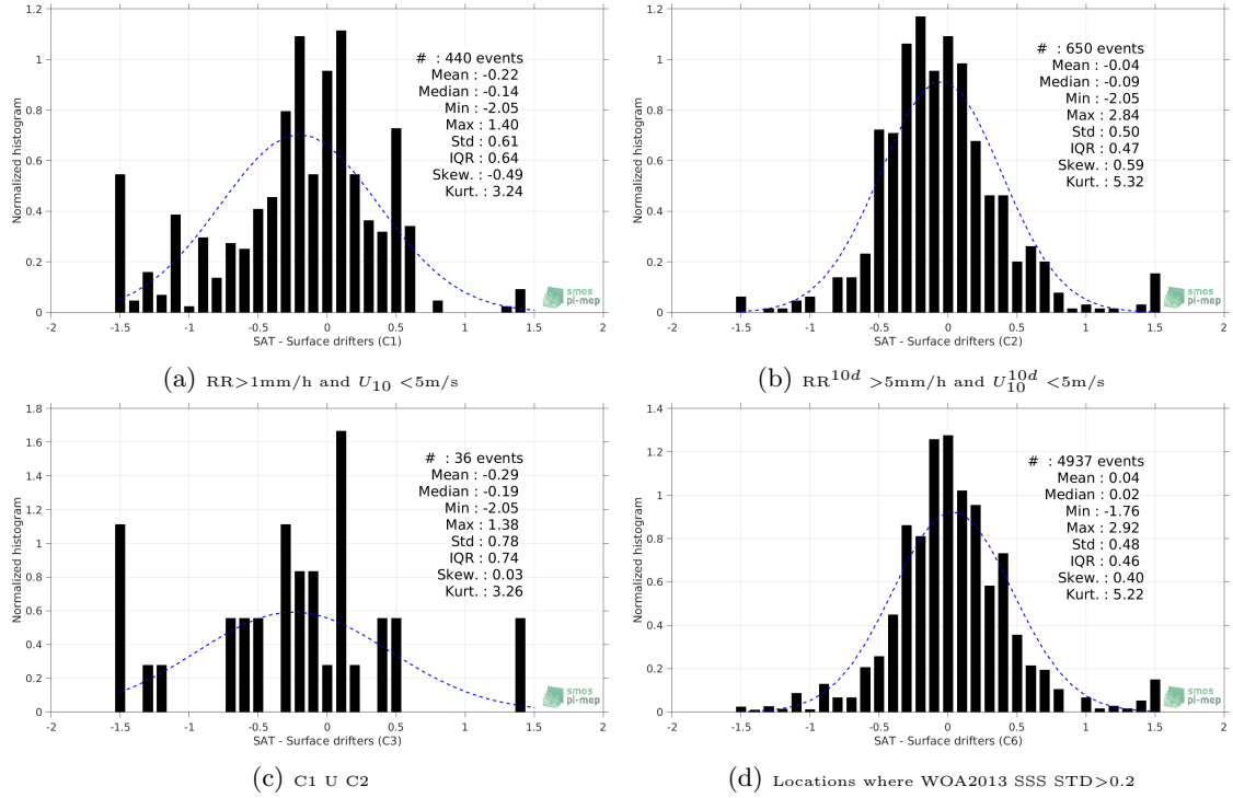
Figure 12: Normalized histogram of \Delta SSS (Aquarius-L2-JPL-V5 - Surface drifters) for 6 different subdatasets corresponding to: RR > 1\text{mm/h} and U_{10} < 5\text{m/s} (a), RR^{10d} > 5\text{mm/h} and U_{10}^{10d} < 5\text{m/s} (b), C1 \cup C2 (c), Locations where WOA2013 SSS STD > 0.2 (d).
