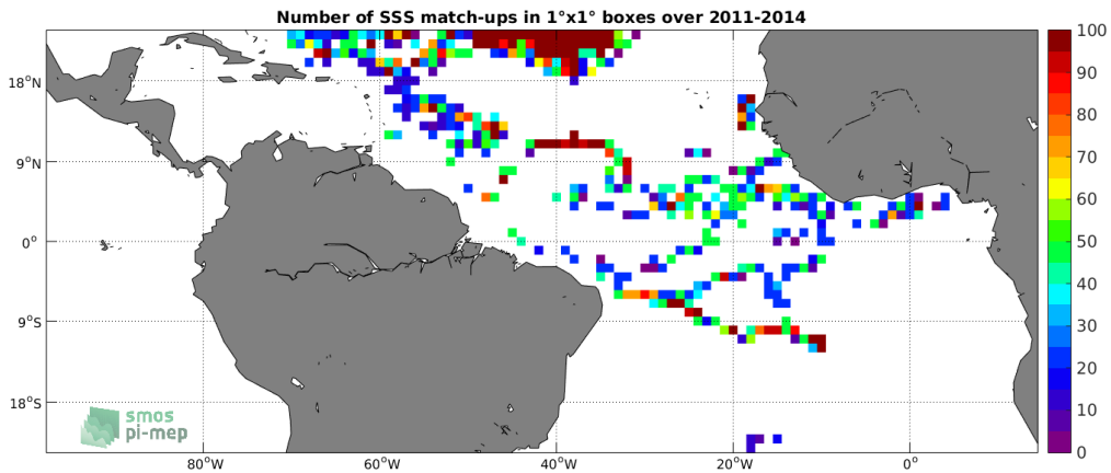
Figure 3: Number of SSS match-ups between Surface drifters SSS and the Aquarius-L2-JPL-V5 SSS product for the Tropical Atlantic Ocean Pi-MEP region over 1^{\circ} \times 1^{\circ} boxes and for the full satellite product period.
