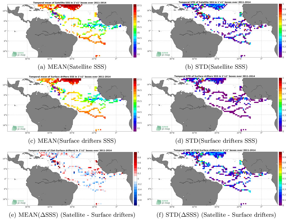
Figure 5: Temporal mean (left) and STD (right) of SSS from Aquarius-L2-JPL-V5 (top), Surface drifters (middle), and of \Delta SSS (Satellite - Surface drifters). Only match-up pairs are used to generate these maps.
