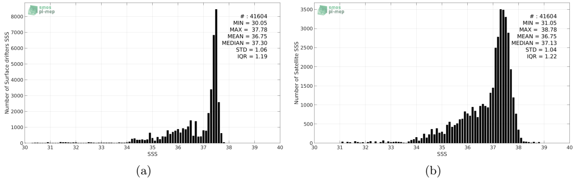
Figure 2: Histograms of SSS from Surface drifters (a) and Aquarius-L2-JPL-V5 (b) considering all match-up pairs per bins of 0.1 over the Tropical Atlantic Ocean Pi-MEP region and for the full satellite product period.
