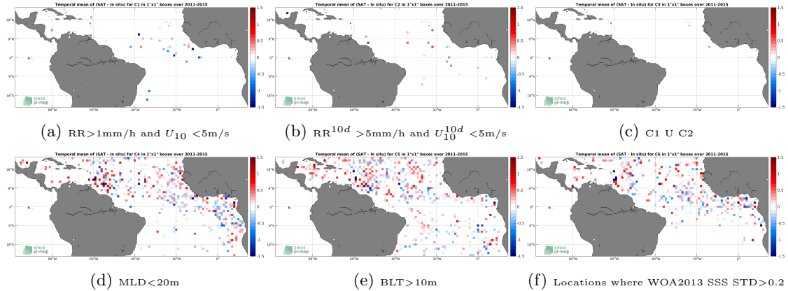
Figure 12: Temporal mean gridded over spatial boxes of size 1^\circ \times 1^\circ of \Delta SSS (Aquarius-L2-JPL-V5 - Argo) for 6 different subdatasets corresponding to: RR > 1\text{mm/h} and U_{10} < 5\text{m/s} (a), RR^{10d} > 5\text{mm/h} and U_{10}^{10d} < 5\text{m/s} (b), C1 U C2 (c), MLD < 20\text{m} (d), BLT > 10\text{m} (e), Locations where WOA2013 SSS STD > 0.2 (f).
