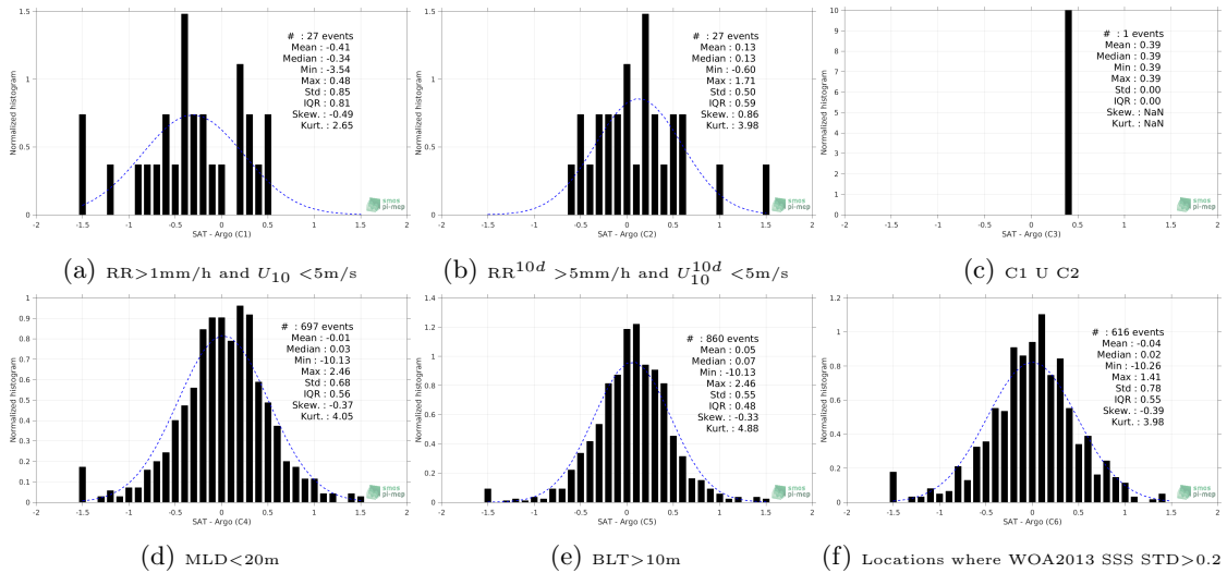
Figure 13: Normalized histogram of \Delta SSS (Aquarius-L2-JPL-V5 - Argo) for 6 different subdatasets corresponding to: RR > 1\text{mm/h} and U_{10} < 5\text{m/s} (a), RR^{10d} > 5\text{mm/h} and U_{10}^{10d} < 5\text{m/s} (b), C1 U C2 (c), MLD < 20\text{m} (d), BLT > 10\text{m} (e), Locations where WOA2013 SSS STD > 0.2 (f).
